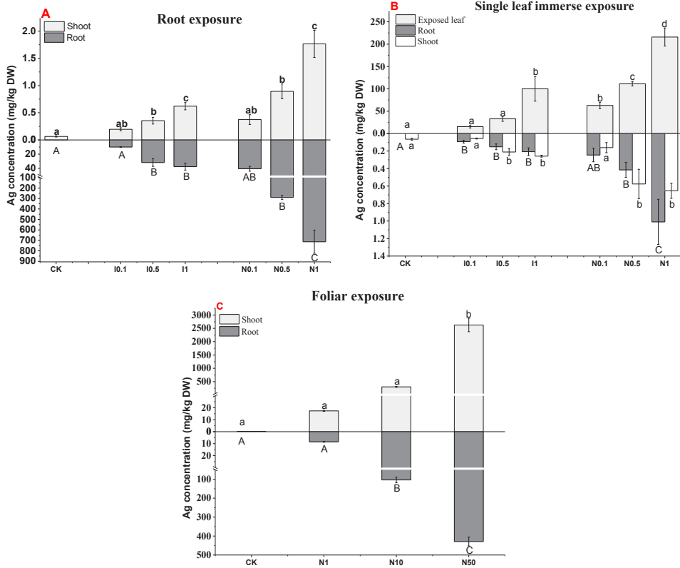
Figure 2.4. Ag concentration in lettuces after exposure to different concentrations of AgNPs and corresponding dissolved Ag + for 15 days. Data are mean \pm SE (n = 4). Within the same plant tissue, the different letters in the same group represent statistically significant differences between the treatments at p < 0.05. I0.1, 0.5 and 1 represent Lactuca sativa exposed to the AgNPs (ion) concentrations as released from AgNPs suspensions with nominal concentrations of 0.1, 0.5 and 1 mg/L; N0.1, 0.5, 1, 10 and 50 represent Lactuca sativa exposed to nominal AgNPs (total) concentrations of 0.1, 0.5, 1, 10 and 50 mg/L.
