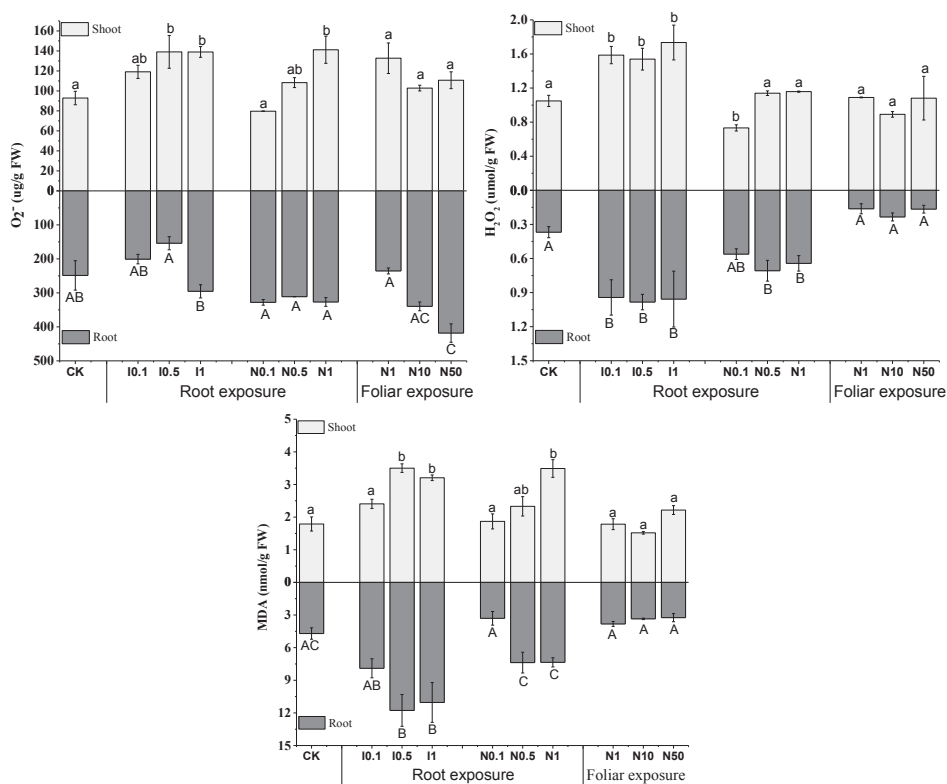
Figure 2.3. O_2^- , H_2O_2 and MDA production in Lactuca sativa exposed to different concentrations of AgNPs_{(total)} and AgNPs_{(ion)} after 15 days of exposure. Data are mean \pm SE (n = 4). Within the same plant tissue, the different letters in the same group indicate statistically significant differences between treatments at p < 0.05 . I0.1, 0.5 and 1 represent Lactuca sativa exposed to the AgNPs_{(ion)} concentrations as released from AgNPs suspensions with nominal concentrations of 0.1, 0.5 and 1 mg/L; N0.1, 0.5, 1, 10 and 50 represent Lactuca sativa exposed to nominal AgNPs_{(total)} concentrations of 0.1, 0.5, 1, 10 and 50 mg/L
