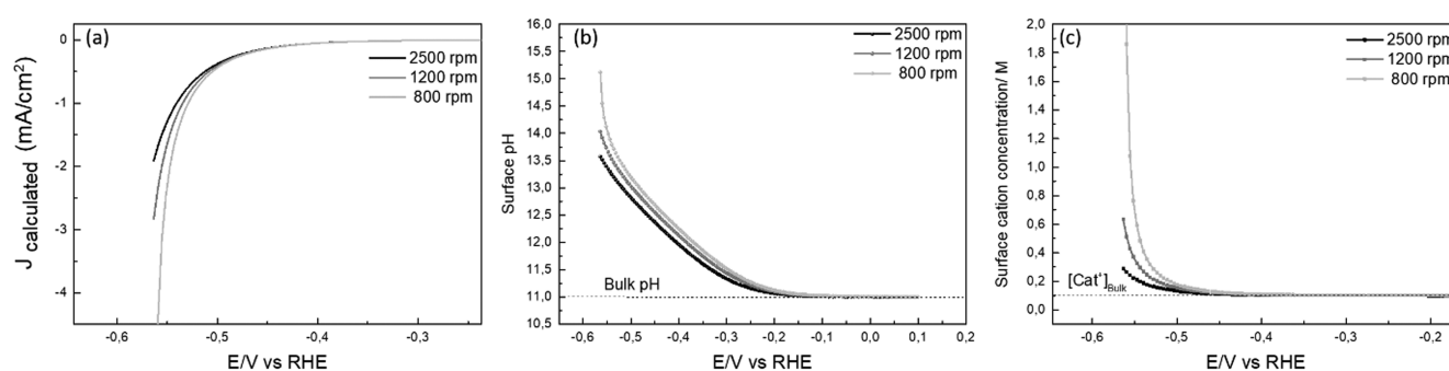
FIG. 6. (a) Simulated linear sweep voltammogram for HER on Au electrodes as obtained from Eq. (S12) (supplementary material) at different rotation rates (2500, 1200, and 800 rpm). (b) The as-calculated surface pH [Eq. (S11)] as a function of the applied overpotential (vs RHE) at different rotation rates, where the bulk pH is 11 in all the calculations. (c) The as-calculated surface cation concentration [Eq. (S7)] as a function of the applied overpotential (vs RHE) at different rotation rates, where the bulk cation concentration is 0.1 M in all the calculations.
