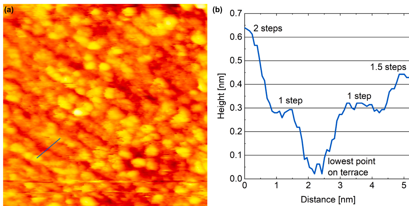
Fig. 5. (a) 35 nm x 35 nm STM image of \text{ZnO}(10\bar{1}0) after 4 h in 1 mbar of water at 400 K with (b) the corresponding height profile indicated in blue. The image is taken in UHV at room temperature with + 4 V and 50 pA. (For interpretation of the references to colour in this figure legend, the reader is referred to the web version of this article.)
