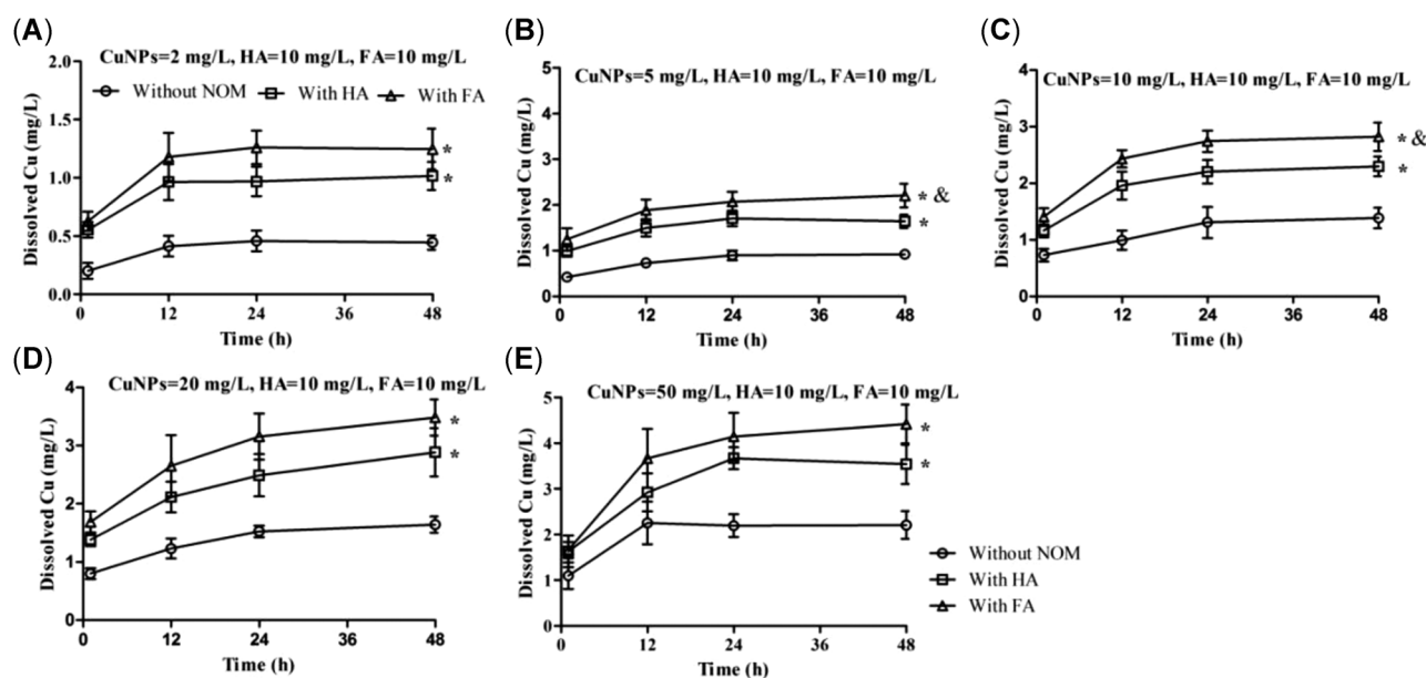
FIGURE 1: Concentration profiles of Cu ion nanoparticles (NP ion ) within 48 hours on different concentrations of Cu NPs and natural organic matter (NOM) treatments. (A–E) Dissolution profiles of Cu NPs with the initial concentrations of 2, 5, 10, 20, and 50 mg/l, respectively. Data are presented as mean \pm standard deviation ( n = 3 ). *Significant difference between treatments with and without the addition of NOM at 48 hours ( p < 0.05 ), **significant difference between treatments of humic acids and fulvic acids ( p < 0.05 ). HA = humic acid; FA = fulvic acid.
