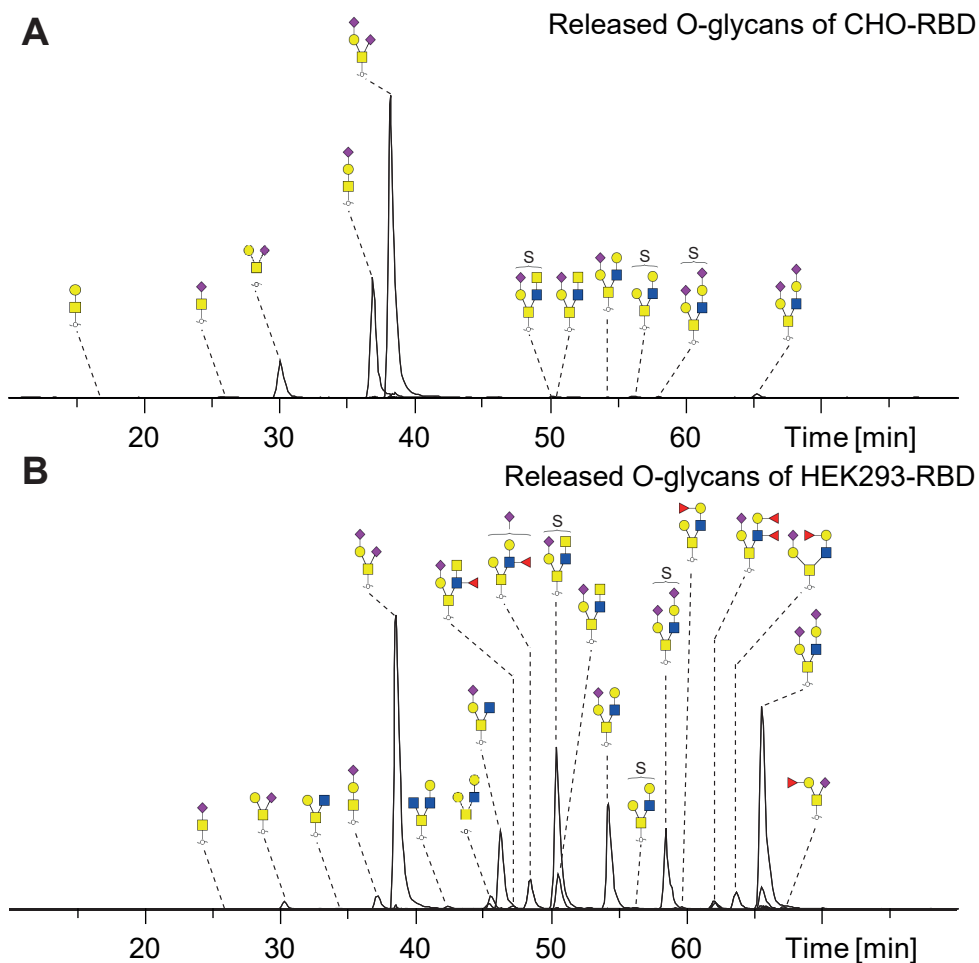
Figure 3. PGC nano-LC-ESI-MS/MS of released O-glycans from A) CHO-RBD and B) HEK2993-RBD. Yellow square, N -acetylgalactosamine; yellow circle, galactose; blue square, N -acetylglucosamine; red triangle, fucose; purple diamond, N -acetylneuraminic acid (sialic acid), S, sulfate.
