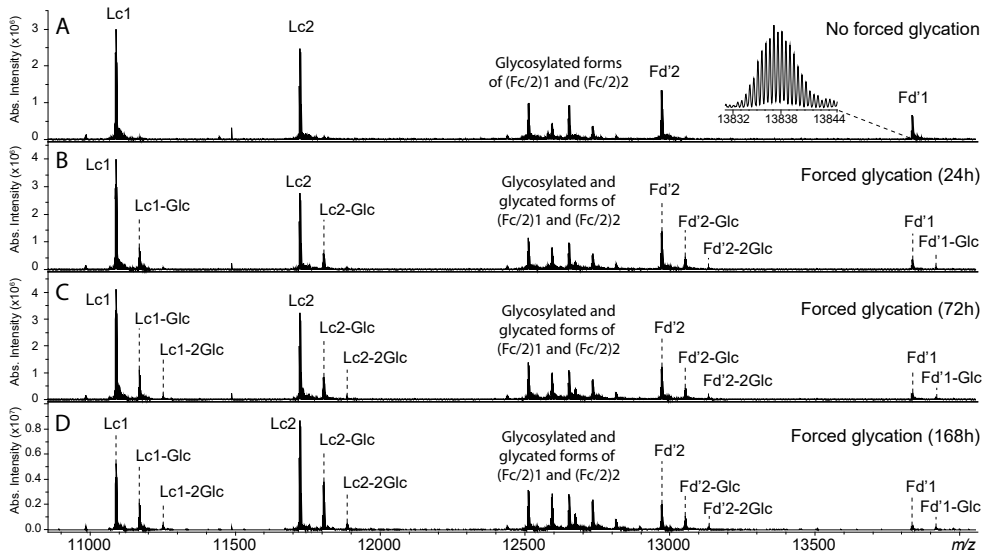
Figure 2. mFT MALDI FT-ICR MS spectra of IdeS-digested and chemically reduced A2V BsAb analyzed (A) prior to and (B-D) after forced glycation. All polypeptide chains, including glycosylated Fc/2 portions, were detected in a single spectrum. Enlargements of such spectra are shown in Figures S1 to S5 .
