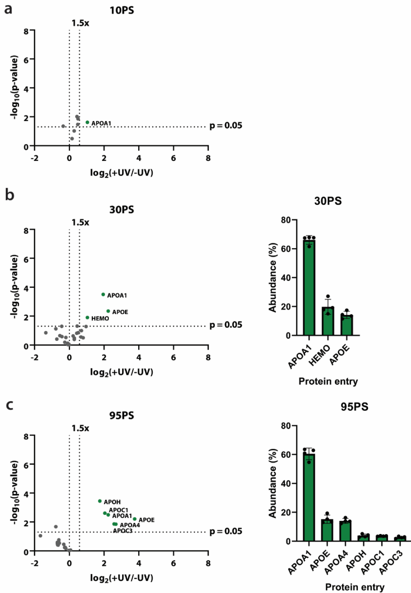
Figure S2. Volcano plots showing the enrichment of proteins in “+UV” over “-UV” samples as \log_2(+\text{UV}/-\text{UV}) against the statistical significance between the two groups ( n \geq 3 ) as -\log_{10}(\text{p-value}) . Selection threshold is set at 1.5fold enrichment and a p-value < 0.05 . Abundance plots only show proteins that meet selection criteria. (a) 10PS (b) 30PS (c) 95PS.
