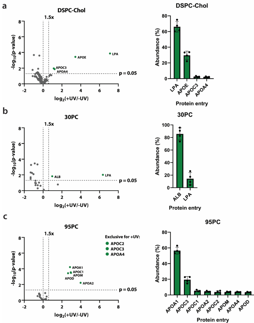
Supplementary Figure 4. Volcano plots showing the enrichment of proteins in “+UV” over “-UV” samples as \log_2(+\text{UV}/-\text{UV}) against the statistical significance between the two groups ( n \geq 3 ) as -\log_{10}(\text{p-value}) . Selection threshold is set at 1.5-fold enrichment and a p-value < 0.05 . Abundance plots only show proteins that meet selection criteria. (a) DSPC-Chol (b) 30PC (c) 95PC.
