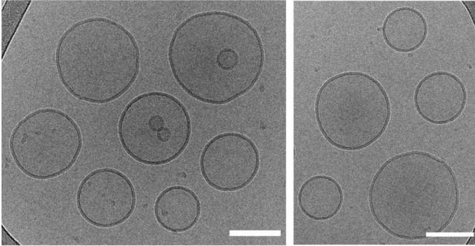
Figure S14. CryoTEM images of anionic LUVs. LUVs are composed of PC:PE:PS:Chol:PI at a ratio of 50:27:10:10:3 mol%. Sample vitrification in the mixture of 100 mM citrate buffer and PBS (1:2 vol:vol) at 37 °C as described in the Materials and Methods section. All scale bars are 100 nm.
