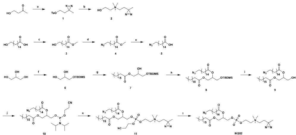
Figure S1. Synthesis scheme of the PAL probe IKSo2. Reagents and conditions: (a) 1. 7N NH 3 in methanol; 2. NH 2 OSO 3 H; 3. I 2 , Et 3 N; 4. TsCl, pyridine, 20% over 4 steps; (b) DMEA, acetone, quant.; (c) AcCl, MeOH, 92%; (d) 1. MsCl, Et 3 N, DCM; 2. NaN 3 , DMF, 70 °C, 91% over 2 steps; (e) 4M NaOH, dioxane, 95%; (f) tBDMSCl, imidazole, DCM:DMF (1:1), -18 °C, 34%; (g) Stearic acid, DCC, DMAP, DCM, 76%; (h) 5, DCC, DMAP, DCM, 64%; (i) Et 3 N·3HF, THF, quant.; (j) PCl(OCH 2 CH 2 CN)(NiPr 2 ), Et 3 N, DCM, 74%; (k) 1. 2, imidazole, DCM; 2. tBuOOH, DCM, 10% over 2 steps; (l) tBuNH 2 , DCM, 48%. Detailed procedures are described in the Chemical Synthesis section of the Supplementary Information.
