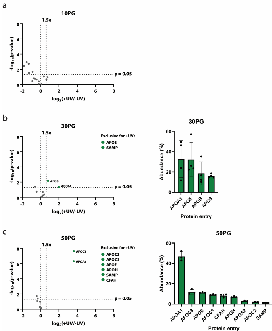
Figure S1. Volcano plots showing the enrichment of proteins in “+UV” over “-UV” samples as \log_2(+UV/-UV) against the statistical significance between the two groups ( n \geq 3 ) as -\log_{10}(p\text{-value}) . Selection threshold is set at 1.5-fold enrichment and a p\text{-value} < 0.05 . Abundance plots only show proteins that meet selection criteria. (a) 10PG (b) 30PG (c) 50PG.
