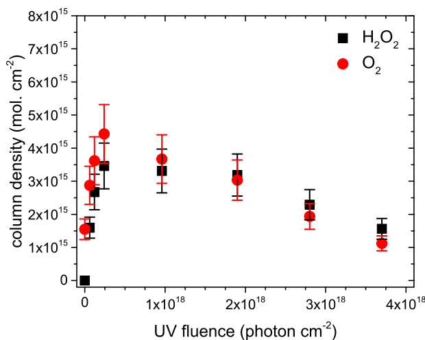
Figure 6.11: Absolute molecular abundances of species during the UV photolysis of mixed ices: \text{H}_2\text{O}:\text{CO}_2:\text{O}_2 ice at 100:22:2 ratio. Initial ice thickness is (90 \pm 10) ML.
