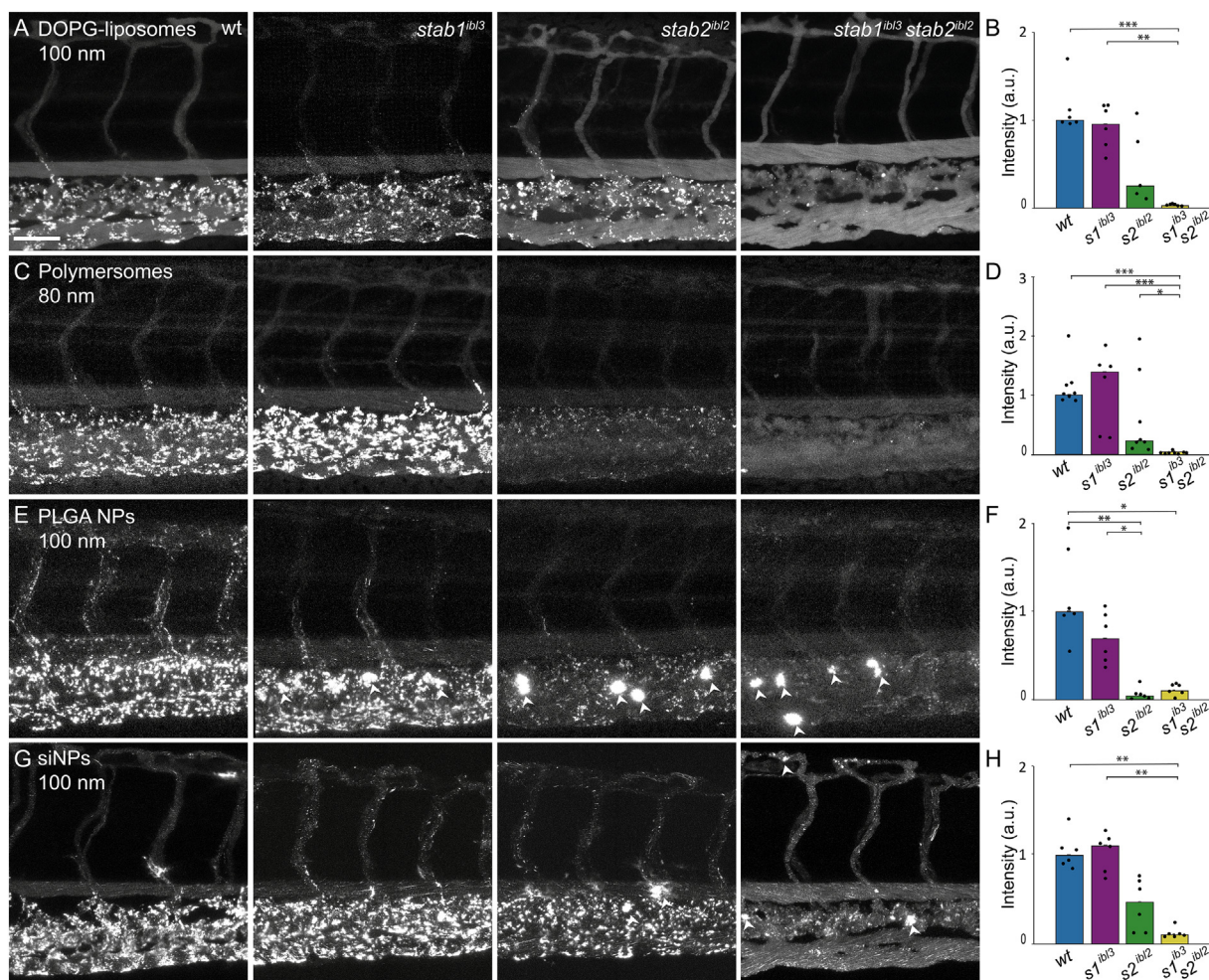
Figure 3. Combined contribution of Stabilin-1 and Stabilin-2 in the clearance of anionic NPs. (A–B) Tissue level view (40×) and quantification of fluorescently labeled DOPG-liposomes, (C–D) polymersomes, (E–F) PLGA NPs, (G–H) siNPs after i.v. injection (1 nL) in wt (AB/TL), stab1 ib13 , stab2 ib12 single and stab1 ib13 stab2 ib12 double mutants at 1–1.5 h post injection (hpi). White arrows indicate apparent NP uptake within plasma-exposed macrophages. Scale bar: 50 μm. Graphs represent intensity of fluorescent NPs in wt and stab mutants. Bar height represents median values, dots are individual data points, and brackets indicate significant values (* P 0.05, ** P 0.01, *** P 0.001) based on Kruskal–Wallis tests followed by two-tailed Dunn’s tests with Bonferroni correction.
