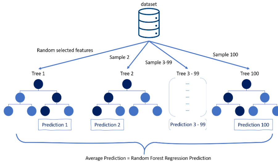
Fig.4: Random Forest Regression Model
