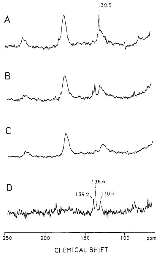
FIGURE 2: MAS NMR spectra of isorhodopsin (A) and a mixture of bathorhodopsin and isorhodopsin (B) containing 8\text{-}^{13}\text{C} retinal. A difference spectrum (D) between spectrum B and a spectrum of unlabeled isorhodopsin (C) yields the spectrum of the 8\text{-}^{13}\text{C} label alone. The spinning speed was 2.5 kHz.
