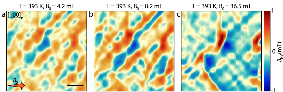
Figure 7.6: Effect of a magnetic field along the easy axis. (a-c) Magnetic field maps with the in-plane component of the bias field along the easy axis ([100] FeRh direction) for T = 393 K. Increasing the bias field does not produce a visible reorientation of domain walls. In (c), some features are more pronounced, but the shape of the domains is qualitatively similar. Scale bar, 20 \mu\text{m} .
