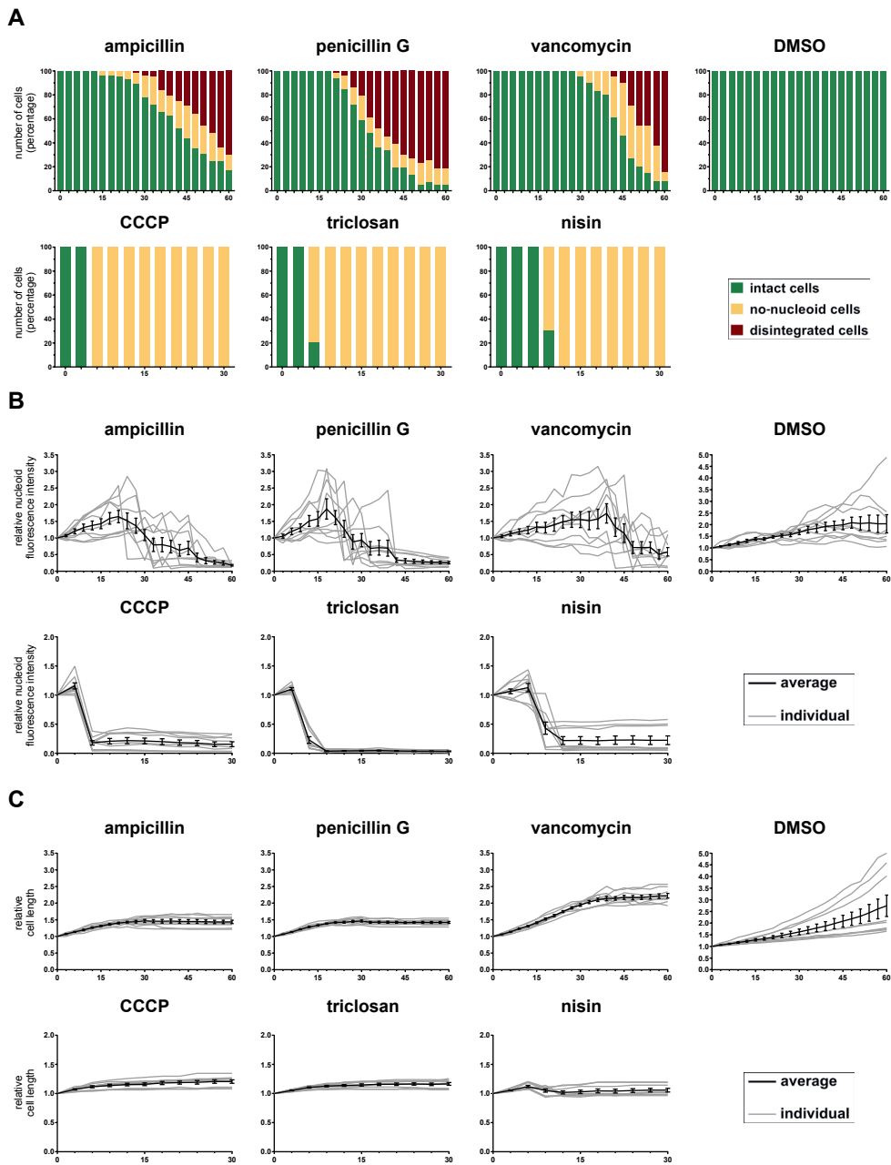
Fig. 5. DBCP of cells treated with antimicrobials from the cell membrane and cell wall classes. B. subtilis cells were treated with antimicrobials ( 2.5 \times \text{MIC} ) as indicated or 1% DMSO (control). Cells were stained with FM4-64 (red, cell membrane) and SYTO-9 (green, nucleoid), and imaged by time lapse confocal fluorescence microscopy with 3 min intervals. Three distinct cell types were identified: intact cells (cells with visible membrane and nucleoid fluorescence), no-nucleoid cells (cells with
