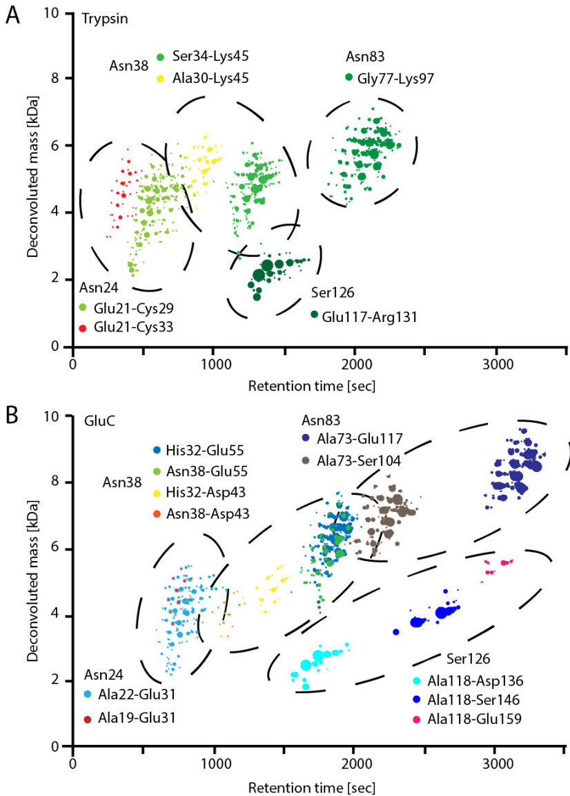
Figure 3.1: Visualization of detected rhEPO glycopeptides in representative replicates by RP-LC-MS/MS analysis upon (A) trypsin digestion after aminoethylation and (B) GluC digestion after carboxymethylation. Glycopeptide assignment and visualization was performed using GlycopeptideGraphMS [89]. The diameter of the data points indicate the relative abundance of the glycopeptides (logarithmic scaling between intensities from 1 \times 10^6 to 1 \times 10^{12} ). Data points with the same color have the same peptide backbone but different glycan compositions.
