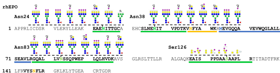
Figure 3.3: Sequence of rhEPO. Tryptic peptides covering glycosylation sites (green) and relevant deamidation (orange) and oxidation sites (blue) are highlighted. For the glycosylation sites, the eight most abundant glycoforms are presented. Structural ambiguities of the glycoforms were reduced by information from the literature [77].
