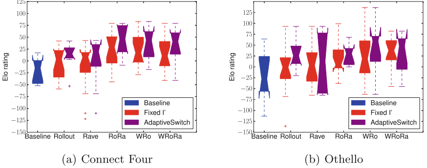
Fig. 2. Comparison of adaptive switch method versus fixed I' based on a full tournament for 6 \times 6 Connect Four and Othello
