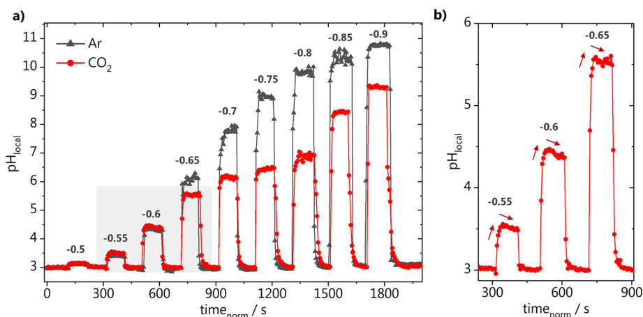
Figure 3. Local pH measured in time. (a) Comparison of the pH measured at the same distance from the surface in argon and CO 2 atmospheres; (b) inset of the shaded area of panel a showing the pH trend at low overpotentials. The sample potentials are indicated on top of the curves, in V vs Ag/AgCl.
