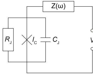
Figure 2.3: Circuit diagram of a Josephson junction in STM. The Josephson junction with maximum critical supercurrent I_C is biased with a voltage V . The junction has a resistance R_J and capacitance C_J . To account for dissipation effects a complex impedance Z(\omega) is connected in series with the junction.
