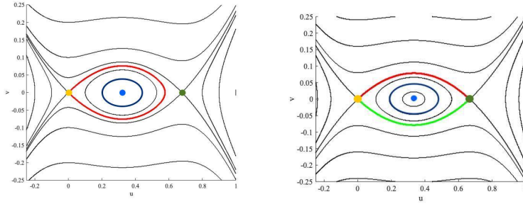
(a) Homoclinic orbit connecting the fixed point (u_0, v_0) to itself for a = \frac{7}{9} + \frac{1}{250} . (b) Heteroclinic orbits connecting the fixed point (u_0, v_0) to the fixed point (u_+, v_0) with a = \frac{7}{9} . Note that due to the symmetry of the system we have two heteroclinic orbits (red and green).
