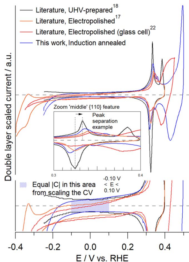
Figure 3. Comparison of literature reported CVs of Cu(110) with an induction annealing-prepared sample. CVs have been manually shifted up/down to reach the maximum amount of symmetry around the x-axis of the main adsorption features. CVs have been scaled to the absolute charge of the CV region represented by the blue dotted box, with the potential boundaries as specified in the image.
