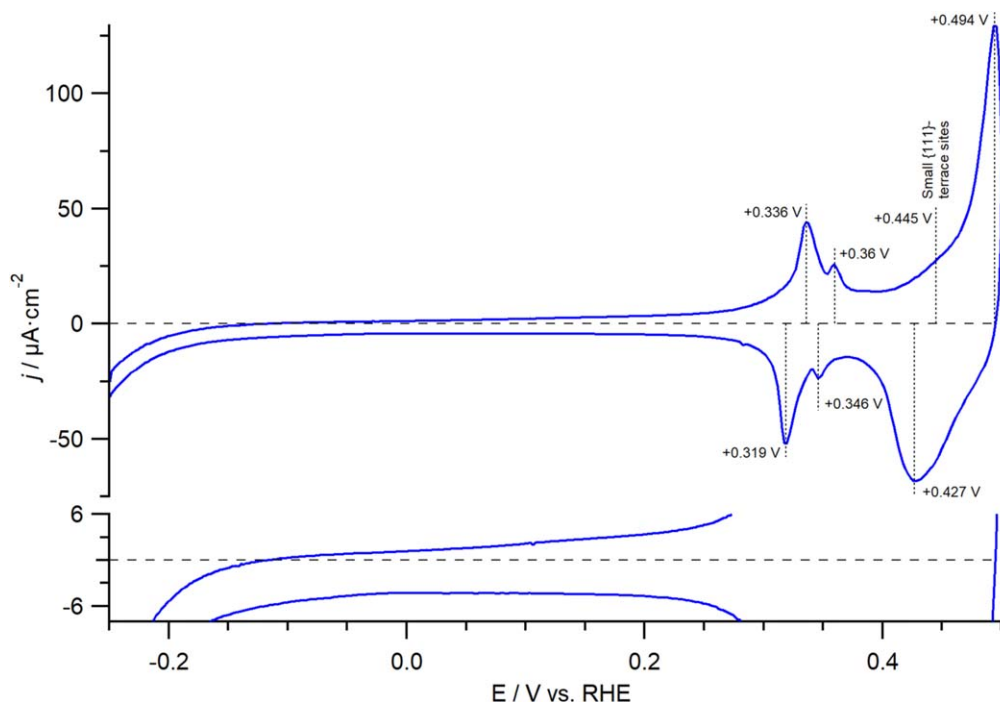
Figure 6. Normalized (geometric area) CV of Cu(110) as obtained after preparation via induction annealing, employing the electrochemical procedure described in the experimental section. Measured in 0.1 M NaOH at scan rate = 50 mVs -1 .
