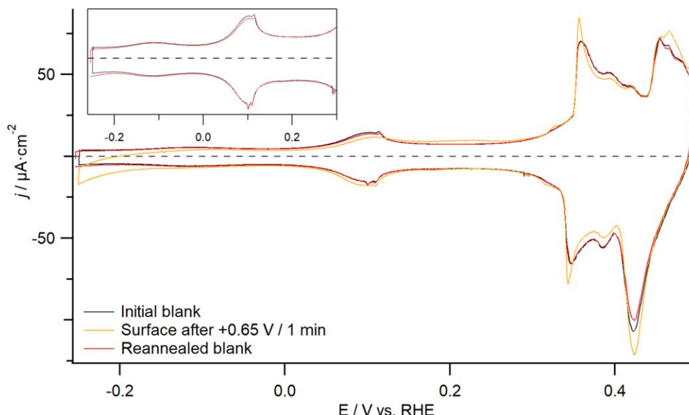
Figure 8. Illustration of the reproducibility of a polycrystalline surface after having been regenerated via induction annealing-treatment. In black, the initially obtained CV is depicted, whereas in orange the state of the surface is depicted after having been oxidized at +0.65 V for 60 s in 10 M NaOH. In red, the surface has been reannealed to recover its initial state. All CVs were measured in 0.1 M NaOH at scan rate = 50 mVs -1 .
