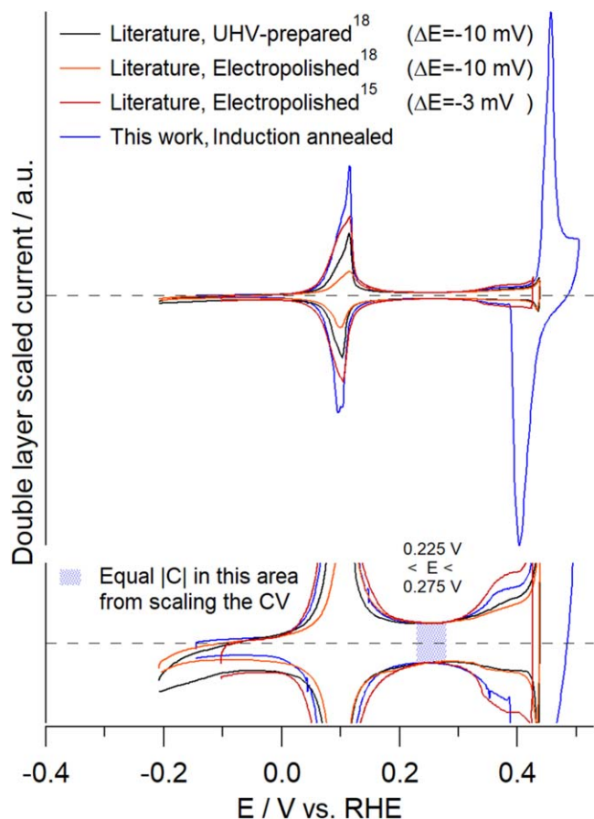
Figure 1. Comparison of literature reported CVs of Cu(111) with an induction annealing-prepared sample. CVs have been manually shifted up/down to reach the maximum amount of symmetry around the x -axis of the main adsorption features. CVs have been scaled to the absolute charge of the CV region represented by the blue dotted box, with the potential boundaries as specified in the image. \Delta E values represent the amount by which literature CVs were manually adjusted to align the key adsorption feature at +0.1 V with the induction annealed CV.
