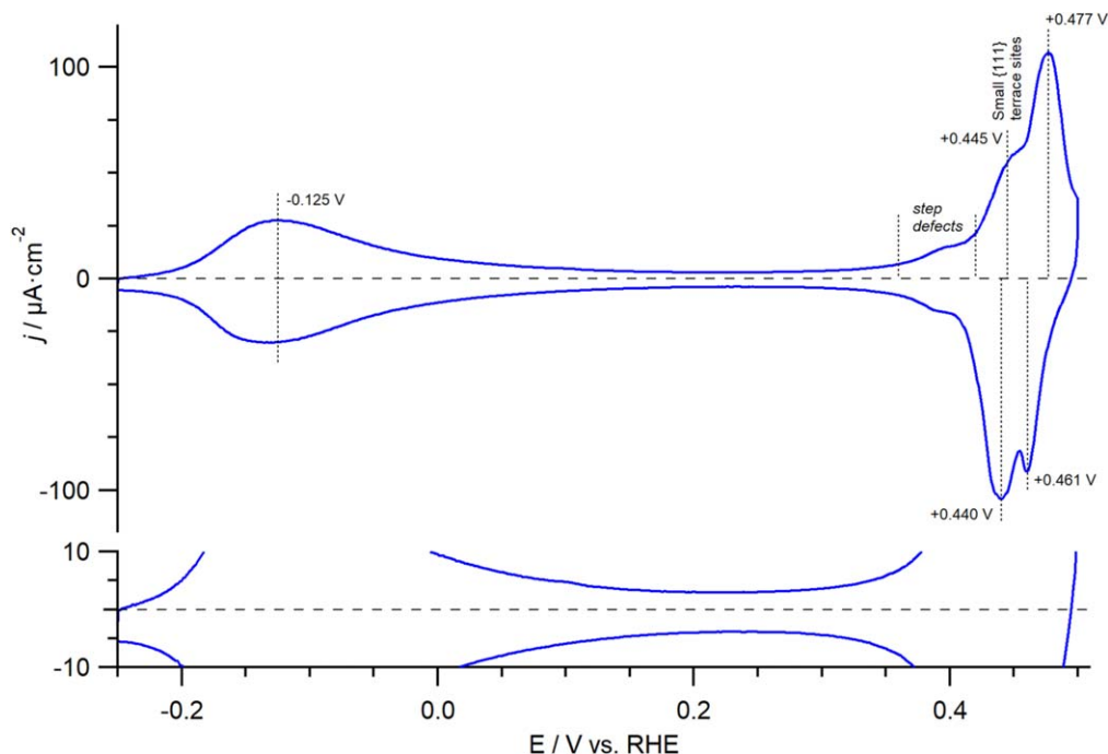
Figure 5. Normalized (geometric area) CV of Cu(100) as obtained after preparation via induction annealing, employing the electrochemical procedure described in the experimental section. Measured in 0.1 M NaOH at scan rate = 50 mVs -1 .
