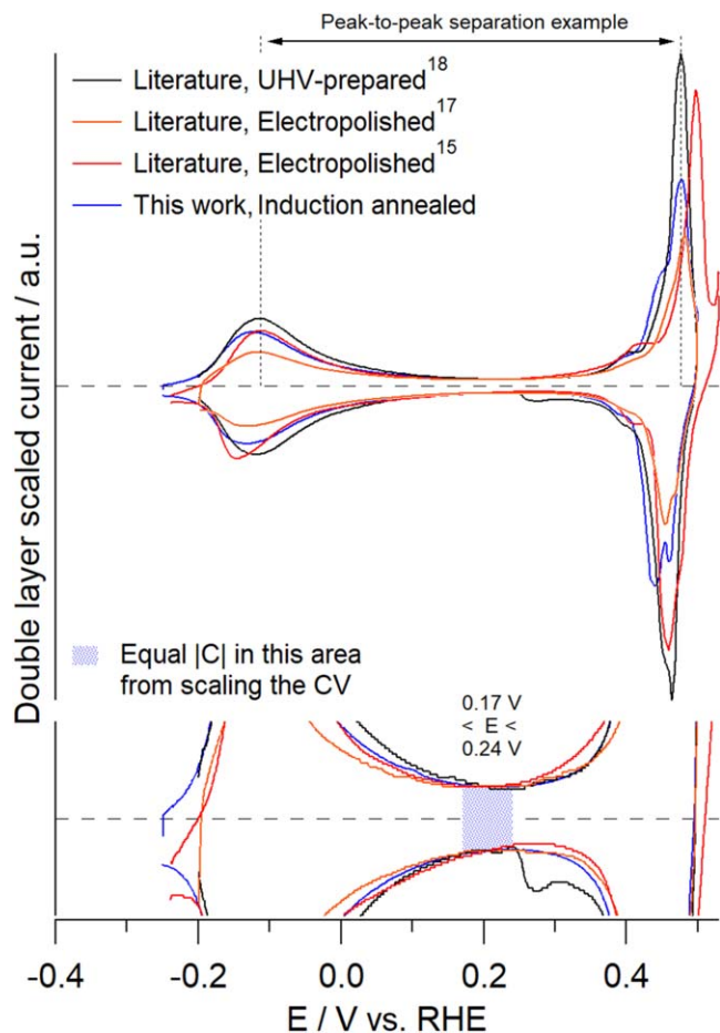
Figure 2. Comparison of literature reported CVs of Cu(100) with an induction annealing-prepared sample. CVs have been manually shifted up/down to reach the maximum amount of symmetry around the x -axis of the main adsorption features. CVs have been scaled to the absolute charge of the CV region represented by the blue dotted box, with the potential boundaries as specified in the image.
