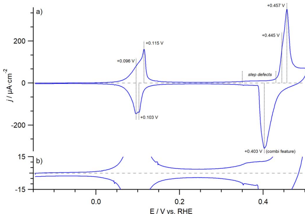
Figure 4. Normalized (geometric area) CV of Cu(111) as obtained after preparation via induction annealing, employing the electrochemical procedure described in the experimental section. Measured in 0.1 M NaOH at scan rate = 50 mVs -1 .
