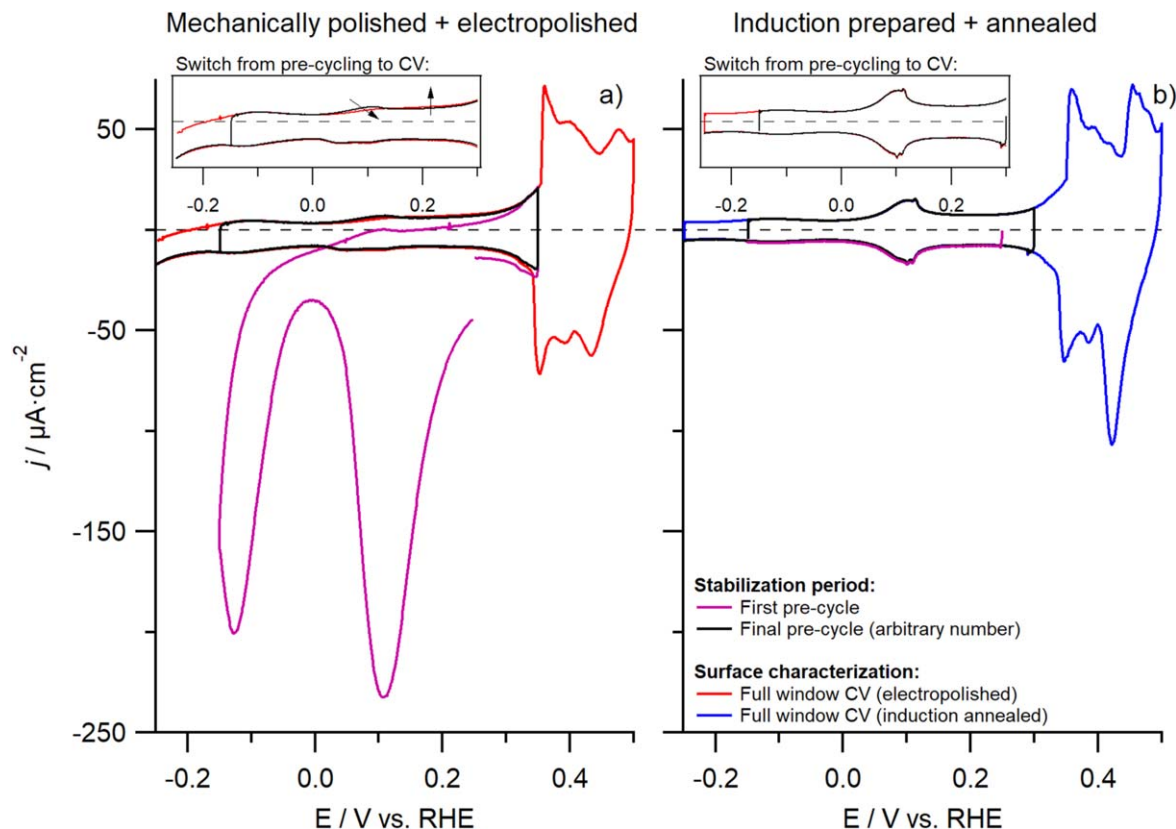
Figure 7. Typical copper CV ( 0.1\text{ M NaOH} , scan rate = 50\text{ mVs}^{-1} ) obtained after a) mechanical polishing + electropolishing treatment and b) induction annealing treatment. In purple, the first CV after establishing electrolyte contact is depicted, while the last pre-characterization cycle (i.e., initial cycling in a smaller potential window to stabilize the surface and remove oxygen) is depicted in black. In red and blue are shown the full-window characterization CVs for the electropolished and induction annealing-prepared surfaces, respectively.
