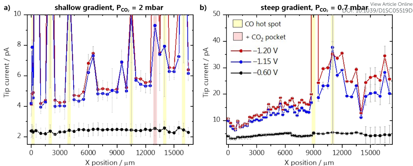
Fig. 3 SECM array scans along a) the catalyst gradient of GDE-A at a \text{CO}_2 back-pressure of 2 mbar, and b) the steep gradient of GDE-B at a \text{CO}_2 pressure of 0.7 mbar. The potentials applied to the GDEs were -1.2 V (red), -1.15 V (blue) and -0.6 V (black) vs. \text{Ag}/\text{AgCl}/3 M \text{KCl} in 1 M \text{KHCO}_3 as electrolyte. \text{CO} hot spots and \text{CO}_2 pockets are marked with a yellow and red shade, respectively.
