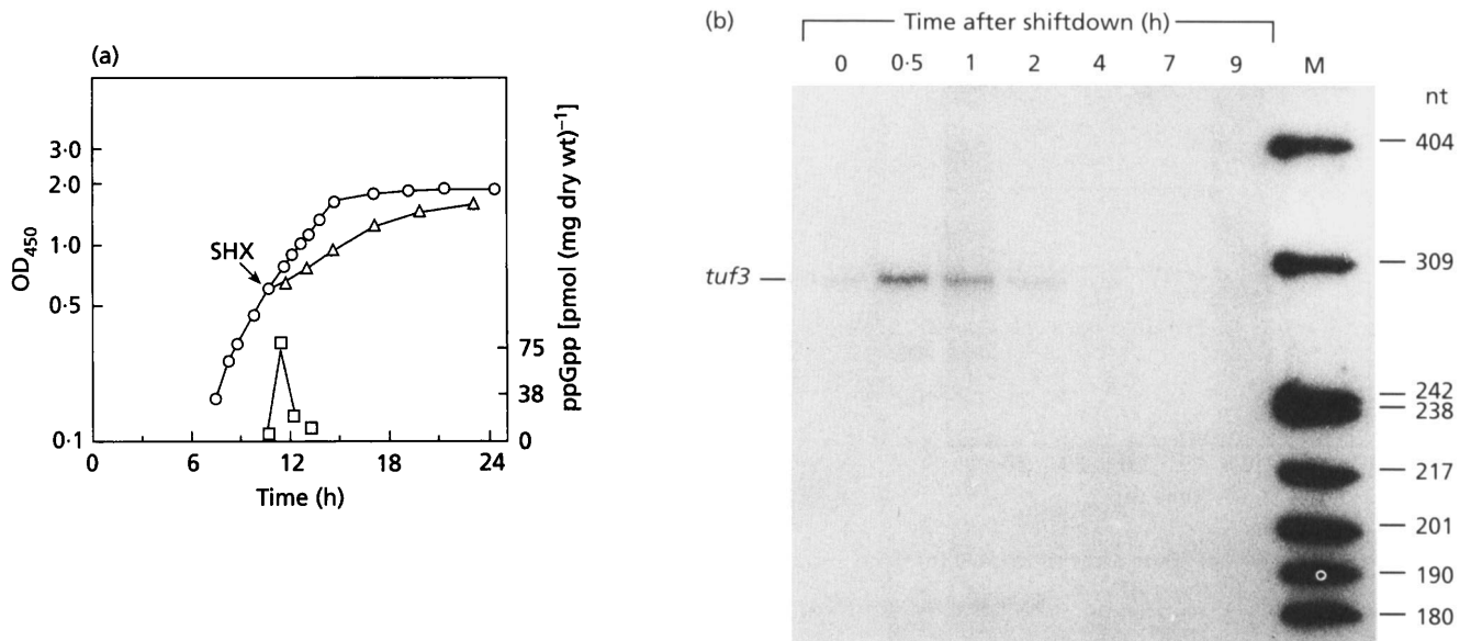
Fig. 8. (a) Growth curve (○, △) and ppGpp production (□) by S. coelicolor M145 in SMM, in the absence (○) or presence (△) of 25 mM SHX. 'SHX' indicates time point of addition of SHX (OD 450 0.6). ppGpp levels were only measured in the SHX-treated culture. (b) Transcription of tuf3 after addition of 25 mM SHX. M, DNA size marker as in Fig. 3.
