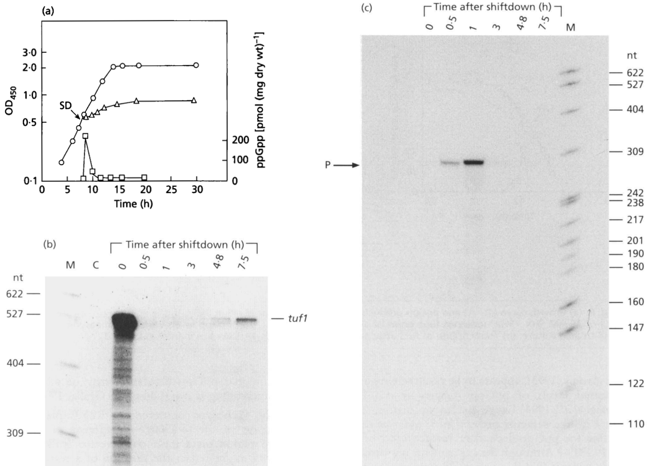
Fig. 7. Transcription of tuf1 and tuf3 after nutritional shiftdown of S. coelicolor M145. (a) Growth curve ( \Delta , \circ ) and ppGpp production ( \square ) of a SMM-grown culture, with ( \Delta ) and without ( \circ ) nutritional shiftdown (SD) at an OD 450 of 0.6. (b) Transcription of tuf1 after nutritional shiftdown. (c) Transcription of tuf3 after shiftdown. P, tuf3 transcripts initiated at the tuf3 promoter around nt position -195; M, DNA size marker as in Fig. 3; C, control lane (30 \mu g tRNA).
