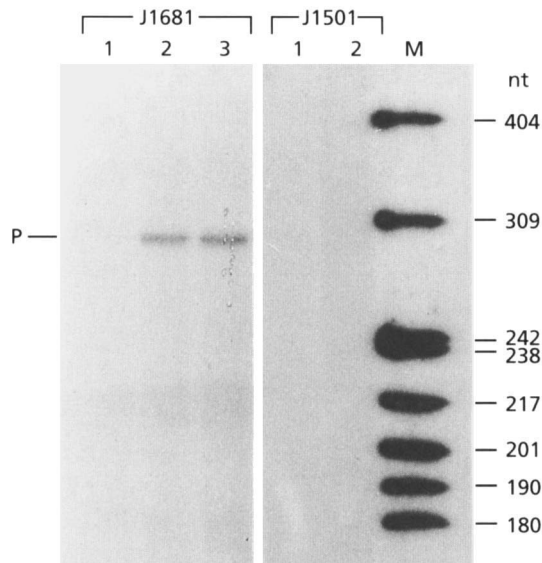
Fig. 6. Transcription of tuf3 in J1501 and J1681 (a bldA deletion mutant of J1501). P, tuf3 transcript. Lanes: M, DNA size marker as in Fig. 3; J1681, RNA isolated from J1681 (J1501 \Delta bldA ) during (1) exponential phase, (2) transition phase and (3) stationary phase; J1501, RNA isolated from J1501 during (1) transition phase and (2) stationary phase.
