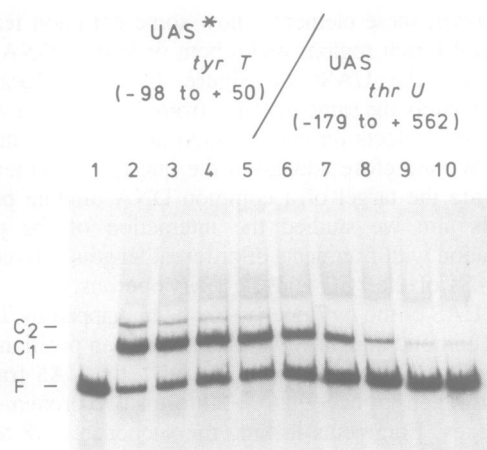
Fig. 6. Competition between UAS fragments of the tyrT and the thrU(tufB) operons for FIS binding. 0.3 nM ^{32} P-labelled UAS fragment of tyrT was incubated with 3 \mu M of the EF-Tu.GDP preparation and the following amounts of unlabeled UAS fragments of the thrU(tufB) (fragment lengths as indicated) in lanes 2–10: 0 nM; 0.35 nM; 0.7 nM; 1.75 nM; 3.5 nM; 7 nM; 17.5 nM; 35 nM, 70 nM, respectively. Lane 1: no protein added.
