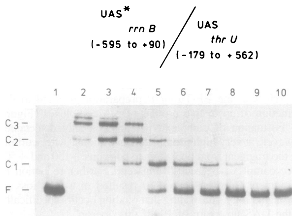
Fig. 7. Competition between UAS fragments of the rrnB and the thrU(tufB) operons for FIS binding. 0.3 nM ^{32} P-labelled UAS fragment of rrnB was incubated with 1.5 \mu M of the EF-Tu.GDP preparation and the following amounts of unlabeled UAS fragments of the thrU(tufB) (fragment lengths as indicated) in lanes 2–10: 0 nM; 0.35 nM; 0.7 nM; 1.75 nM; 3.5 nM; 7 nM; 17.5 nM; 35 nM; 70 nM, respectively. Lane 1: no protein added.
