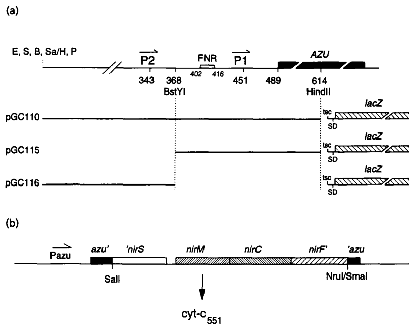
Fig. 1. (a) Promoter-probe constructs in pQF130 (for details see Methods). The complete azu promoter region Hind III– Hind III (pGC110), P1 Bst YI– Hind III (pGC115) and P2 Hind III– Bst YI (pGC116) were cloned upstream of the lacZ gene of pQF130. The lacZ gene is preceded by a ribosome-binding site (SD) and translational stop codons (tsc). Relevant restriction sites are indicated. The restriction sites in the multiple cloning site of pQF130 are Eco RI (E), Sma I (S), Bam HI (B), Sal I/ Hind III (Sa/H) and Pst I (P). (b) The Sal I– Nru I fragment of pEMBL18NR (Silvestrini et al. , 1989) was ligated in Sal I/ Sma I-digested pGC135 (a pUCP24 derivative containing the Pst I azu fragment of pGC13), resulting in pGC139. The promoter region and the first 42 amino acids (including the leader sequence) of azurin are fused in-frame to the C-terminal 107 aa of nitrite reductase ( nirS ). The construct also includes the complete ORF of nirC , a monohaem cytochrome c of unknown function and the N-terminal part of nirF . The product of nirF is suggested to take part in the biosynthetic pathway of haem d , (Kawasaki et al. , 1995).
