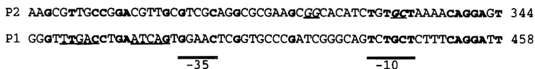
Fig. 4. Nucleotides are numbered according to Houtink et al. (1990). Transcription start sites are at T(344) and T(458). From the data in the paper by Arvidsson et al. (1989) it is difficult to determine the start site of the P1 promoter. The authors indicate position T(457), but the present alignment on the basis of sequence homology shows that T(458) is more likely. The top sequence is the region upstream of the P2 start site and the bottom sequence is upstream of the P1 start site. Identical bases are in bold face. The 'FNR-binding sequence' upstream of the -35 region of P1 is underlined. The GG and GC motifs in the P2 promoter region are in italics and underlined.
