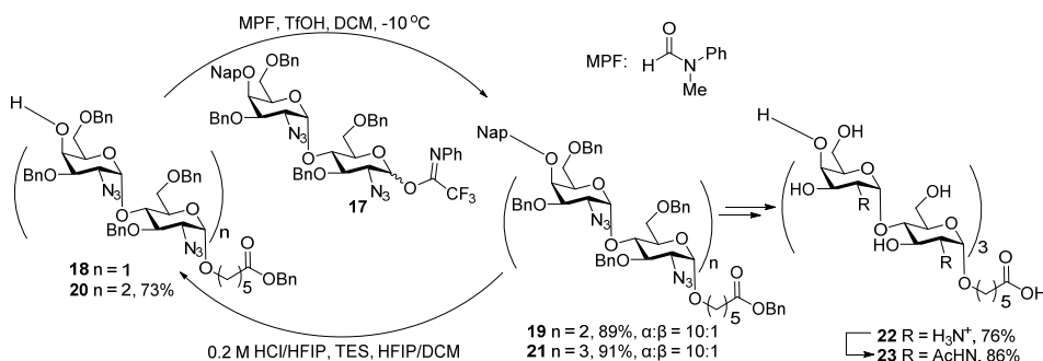
Scheme 2. Chemical synthesis of well-defined Pel oligosaccharides.
