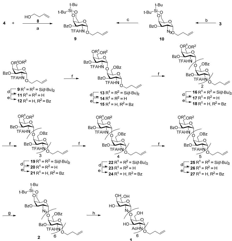
Scheme 2. Synthesis of azido-GAG 1 . a) TFAH, DCM, 3 Å MS, -40 °C, 91% ( \alpha/\beta = 3.2/1 ). b) 8 , TFAH, DCM, 3 Å MS, 0 °C, 86%; c) i) PPh 3 , H 2 O, pyridine, THF ii) TFA 2 O, pyridine, 83%. d) HF/pyridine, THF, yields for 11 : 89%; for 14 : 90%; for 17 : 90%; for 20 : 88%; for 23 : 96%; for 26 : 84%. e) BzOBt, Et 3 N, DCM, yields for 12 : 97%; for 15 : 80%; for 18 : 96%; for 21 : 94%; for 24 : 84%; for 27 : 91%. f) 4 , TFAH, DCM, 3 Å MS, 0 °C, yields for 13 : 86%; for 16 : 75%; for 19 : 84%; for 22 : 68%; for 25 : 18% (0.05M), 54% (0.2 M). g) 3 , TFAH, DCM, 3 Å MS, 0 °C, 84%. h) i) HF/pyridine, THF; ii) 1M NaOH, THF/MeOH; iii) Ac 2 O, NaHCO 3 , H 2 O, 60%.
