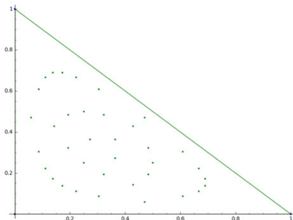
Figure 1. Slice of F_T .
