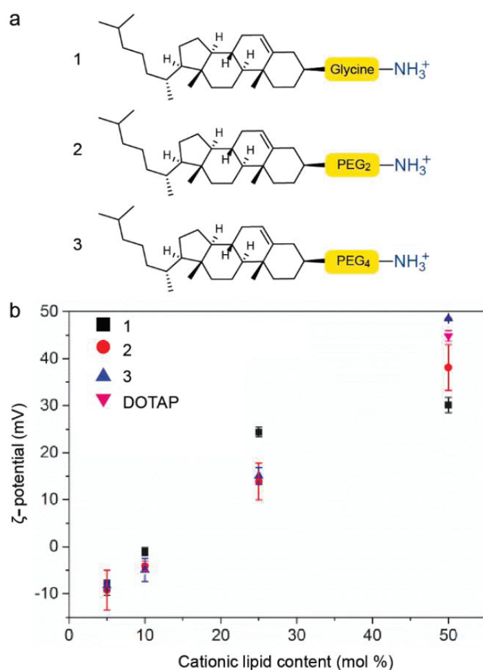
Figure 2. Varying cholesterylamine content within DOPC liposomes. (a) Cationic cholesterylamine analogues, 1-3 . (b) Measured surface charges ( \zeta -potential) of DOPC liposomes containing varying mol% 1-3 . DOPC:DOTAP (1:1) liposomes are included as a representative (commercially available) cationic liposome formulation. Measure of centre: mean; Error bars: standard deviation.
