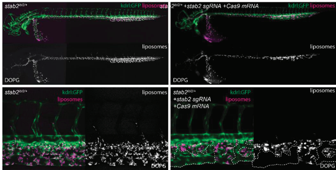
Supplementary Figure 11. Clonal stab2 deletion. Whole-embryo and cellular views of DOPG liposome distribution in stab2 bl2/+ ; kdr1:GFP embryos. CRISPR/Cas9 introduced mutations in the wildtype allele generated clones of cells without stab2 function. In stab2 sgRNA and Cas9 mRNA injected, but not control embryos, endothelial cell clones are observed in which DOPG accumulation is abrogated, indicating a requirement for stab2 function within SECs.
