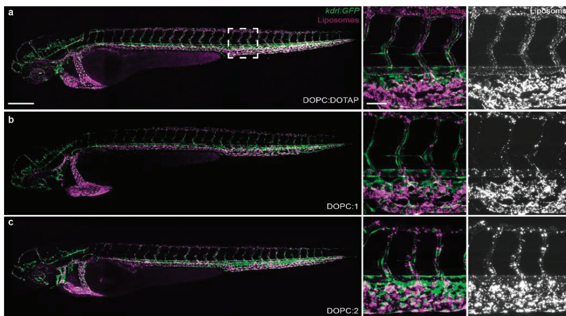
Supplementary Figure 2. Biodistribution of cationic liposomes. Whole embryo and tissue level views of liposome distribution in kdrl:GFP transgenic embryos (2 dpf), 1 hpi of (a) DOPC:DOTAP (1:1), (b) DOPC:1 (1:1) and (c) DOPC:2 (1:1) liposomes. All three cationic liposome formulations are visible as immobile fluorescent punctae associated with blood vessel walls throughout the vasculature of the zebrafish embryo and are largely removed from circulation. Liposomes contained 1 mol% fluorescent lipid probe, DOPE-LR, for visualization. Scale bars: 200 \mu m (whole embryo); 50 \mu m (tissue level).
