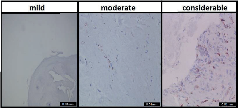
Examples of mild (0-10 macrophages per cm 2 ), moderate (10-100 macrophages per cm 2 ), and considerable (>100 macrophages per cm 2 ) inflammation.
