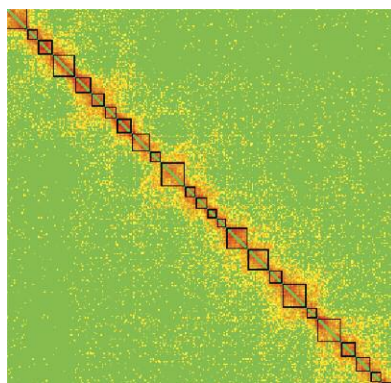
Figure 1: Left: Contact frequency matrix for a segment of the long arm of chromosome 1 ( q from 150.28 Mbp to 179.44 Mbp) from human lymphoblastoid cells GM06990, in logarithmic colour scale. Data from [3]; genomic resolution 100 kbp. The highlighted diagonal blocks define our maximum-resolution TADs. Right: one of our reconstructed structures, consisting of a chain with 292 beads.
