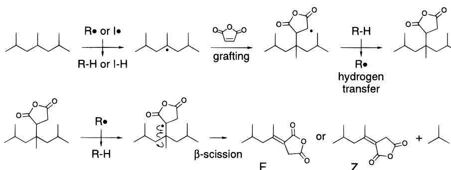
Figure 3. Proposed mechanisms for the grafting of MA onto PE, alt -EPM, and iPP, and onto corresponding structures in copolymers. I• represents an initiator radical, R a polymer chain, and R• a macroradical.
