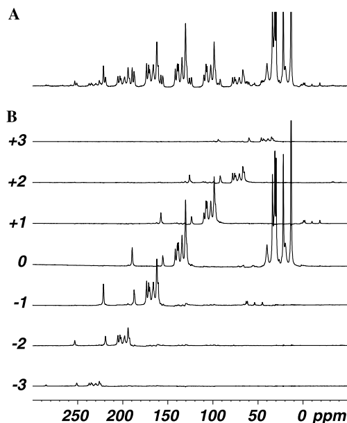
Fig. 2. Experimental results from 2D PASS experiment on U- ^{13}\text{C} -tyrosine-HCl at 750 MHz, 6 kHz spin rate. The corresponding 1D spectrum is shown above.
