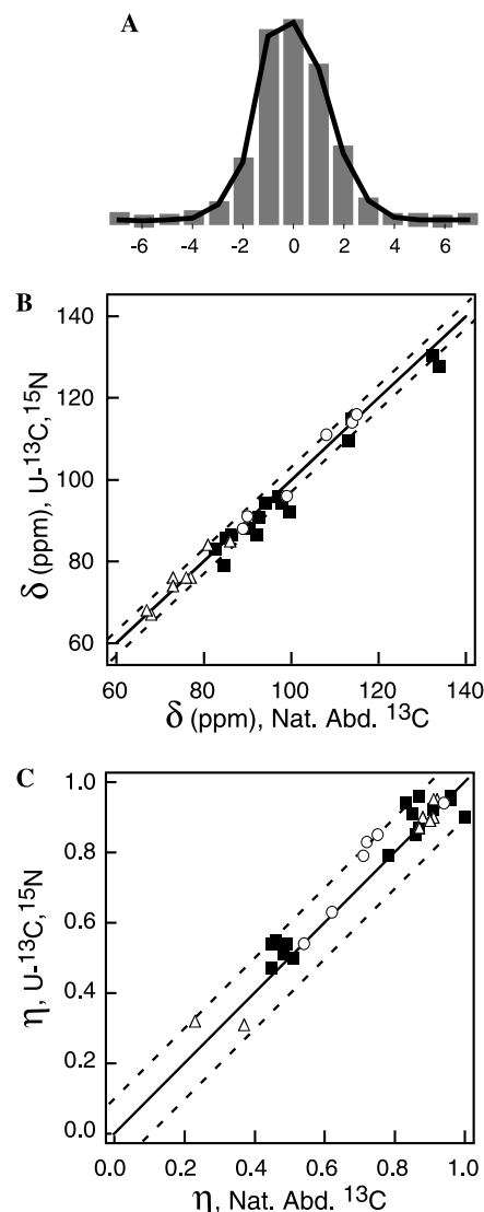
Fig. 3. Fitting and experimental results. Experimental sideband intensities (gray bars) and the best simulated fit (black line) for the C8 position of [U- ^{13}\text{C} ]all-E-retinal are shown in (A). The spin rate was 6 kHz at 188 MHz. The fitting procedure yielded \delta_{\text{aniso}} = -2.72 for both cases, and \eta = 0.85 and 0.86 for the unlabeled and uniformly ^{13}\text{C} labeled systems, respectively. The final \chi^2 was 8.7 ( n = 15 ). (B and C) Correlation plots of experimentally determined \delta and \eta values obtained from natural abundance and uniformly isotopically labeled samples, respectively at spin rates of 4–6.5 kHz. Black squares, retinal; white triangles, histidine-HCl-H _2 O; and white circles, tyrosine-HCl. The solid line represents 1:1 correspondence between the two measurements. The dotted lines represent error limits of \pm 3 ppm and \pm 0.1 in the anisotropy and asymmetry, respectively.
