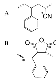
Figure 1. Chemical structure of poly(styrene-co-acrylonitrile) (A) and poly(styrene-co-maleic anhydride) (B). The asterisks indicate the positions of the labels.
