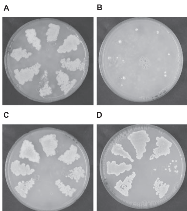
Fig. 1. Lethal effect of MreB overexpression on solid growth. S. coelicolor M145 strains were plated in the absence (A and C) and presence (B and D) of 10 \mu\text{g ml}^{-1} of the inducer thioestrepton. S. coelicolor M145 carrying pPM1 [ tipAp-mreB ] (A and B) and the vector pGM190 (C and D) were streaked onto the plates indicated. Each patch is an independent isolate of the strains.
