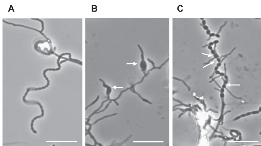
Fig. 4. Effect of mreB deletion on morphological differentiation. S. coelicolor M145 (A) and mreB -IM (B and C) were grown on MS agar for 2–3 days before being prepared for light microscopy. White arrows indicate swollen aerial hyphae (B) and prematurely germinating spores (C) caused by the deletion of mreB . Bar = 10 \mu m.
