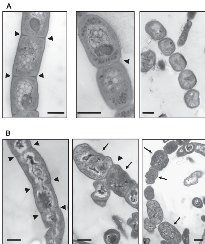
Fig. 5. Transmission electron micrographs of the mreB mutant. Thin sections of sporogenic aerial hyphae of S. coelicolor M145 (A) and its mreB -IM gene replacement mutant (B) were analysed at high resolution by transmission electron microscopy. Left, middle and right panels show prespores, almost mature spores and mature spores respectively. While septation (arrowheads) is not affected by the deletion of mreB , integrity of cell walls is highly compromised, resulting in strongly deformed spores (arrows). Bar = 500 nm.
