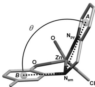
Figure 6. The \theta angle between the pyridine centroid (A), the amine/imine nitrogen atom ( N_{am} ) and the phenol centroid (B) of the coordinated ligand.
