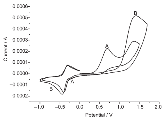
Figure 15. Cyclic voltammograms of 0.001 M Hpyramol (A) and 0.001 M Hpyrimol (B) in DMF, at room temperature, versus Ag/Ag + .
