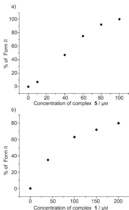
Figure 9. a) Plot of the different concentrations of complex 5 (used to digest \phi X174 phage DNA (20 \mu M)) versus the percentage of Form II formed after 8 h incubation at 37°C. b) Plot of the different concentrations of complex 1 (used to digest \phi X174 phage DNA (20 \mu M)) versus the percentage of Form II formed after 8 h incubation at 37°C.
