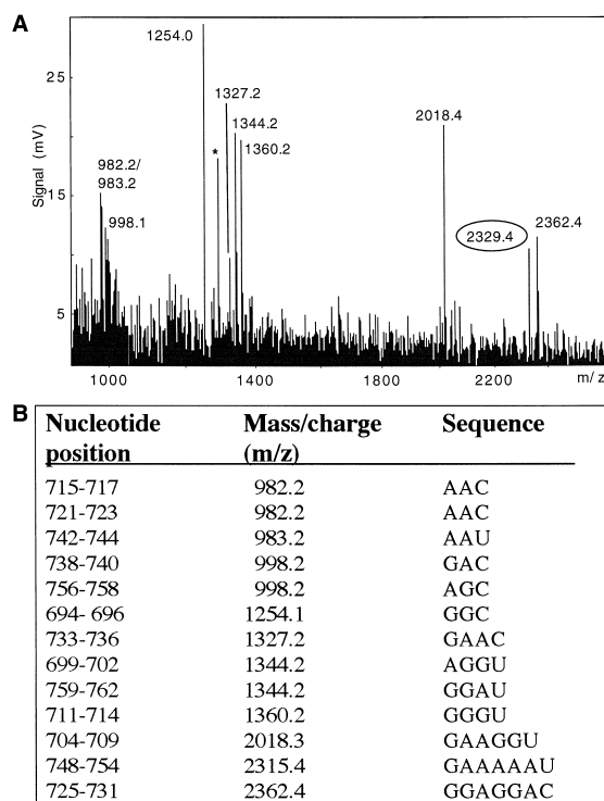
Fig. 4. A. MALDI time-of-flight mass spectrum of the 74-mer RNA after methylation by TlrB and digestion with RNase A. The empirically determined mass/charge (m/z) ratios of the fragments are indicated. The fragment at m/z 2329.4 corresponds to GAAAAAU with a methyl group. The residual unmethylated fragment at m/z 2315.4 disappears into the background noise after TlrB treatment. The fragment at m/z 1254.0 contains the 5'-triphosphate and is therefore prone to form a potassium salt (marked *). B. Table of the fragments predicted after RNase A digestion of the unmodified 74-mer RNA (only trinucleotides and larger are shown). The m/z ratios are calculated for singly protonated fragments that have masses increased by 1.0 Da in comparison with neutral fragments.
