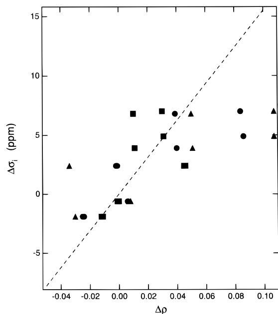
FIGURE 4: Chemical shift differences \Delta\sigma_i versus fractional charge differences \Delta\rho for the doubly charged model structures: (▲) the free structure III , (●) the structure IV stabilized with water molecules, and (■) the structure VI stabilized by monovalent \text{Cl}^- counterions. The dashed line indicates the Spiesecke–Schneider proportionality relation with a 155 ppm shift per unit of charge (Spiesecke & Schneider, 1961).
