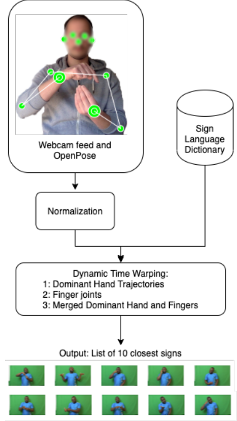
Figure 2: Overview of the overall pipeline of our methodology.
