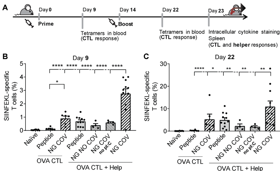
Figure 7. Peptide vaccination with covalently loaded nanogels enhances induction of CTL responses
