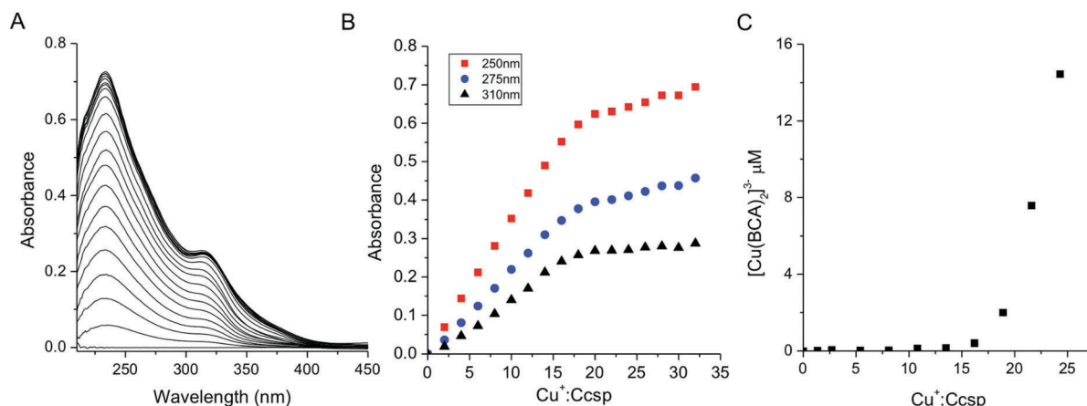
Fig. 3 \text{Cu}^+ ion binding to Ccsp. (A) UV-vis difference spectrum upon titration of \text{Cu}^+ ions to Ccsp (5.6 \mu\text{M} ) showing the appearance of (\text{Cys})\text{S}\gamma \rightarrow \text{Cu}^+ LMCT bands. (B) Plots of absorbance at selected wavelengths taken from (A) versus the \text{Cu}^+:\text{Ccsp} concentration ratio. A break point in the absorbance is reached at \sim 18\text{--}20 \text{Cu}^+ equivalents. (C) A plot of [\text{Cu}(\text{BCA})_2]^{3-} concentration versus the \text{Cu}^+:\text{Ccsp} concentration ratio upon titrating \text{Cu}^+ ions into Ccsp (5 \mu\text{M} ) in the presence of 50 \mu\text{M} BCA. A [\text{Cu}(\text{BCA})_2]^{3-} complex starts to form after the addition of 15 equivalents of \text{Cu}^+ ions. All experiments were performed in 10 mM MOPS pH 7.5, 150 mM NaCl.
