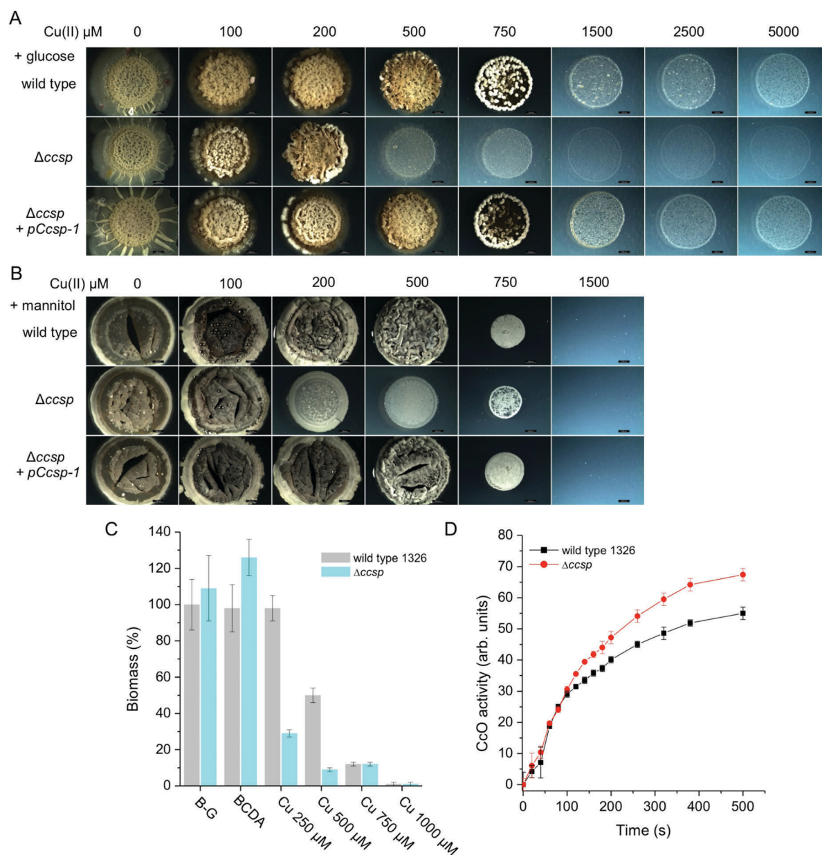
Fig. 6 The effect of Ccsp on the growth and development of S. lividans at 30 °C. Cu tolerance after 6 days growth of the wild type parent strain, the \Delta\text{ccsp} mutant strain and the \Delta\text{ccsp} mutant strain complemented with the pCcsp-1 plasmid on defined agar media with (A) glucose and (B) mannitol as the sole carbon source. Cu(II) concentrations as indicated. All images are the same magnification with a scale bar of 2 mm. (C) Biomass production after 32 h in liquid Bennetts-glucose (B-G) cultures for the wild type and the \Delta\text{ccsp} mutant strain in the presence of the Cu chelator BCDA and various concentrations of Cu(II) citrate. The dry weight biomass of the wild type strain in the B-G culture was set at 100%. (D) CcO oxidase activity at 24 h growth on B-G agar detected by the TMPD assay. Average pixel intensity of the indophenol blue stained mycelium were calculated using ImageJ software 38 and expressed in arbitrary units. Experiments were carried out in triplicate.
