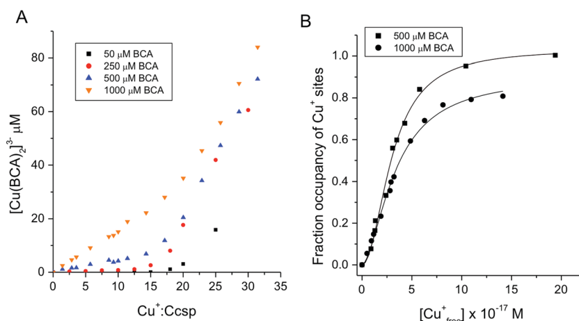
Fig. 4 Affinity of Ccsp for \text{Cu}^+ ions (A) plots of [\text{Cu}(\text{BCA})_2]^{3-} concentration versus the \text{Cu}^+:\text{Ccsp} concentration ratio upon titrating \text{Cu}^+ ions into Ccsp (5–10 \mu\text{M} ) in the presence of different concentrations of BCA as indicated on the plot. As the BCA concentration increases a competition with Ccsp for \text{Cu}^+ ions occur. (B) Plots of fractional occupancy of \text{Cu}^+ binding sites in Ccsp at varying \text{Cu}_{\text{free}}^+ concentrations determined from the data in (A) at 500 and 1000 \mu\text{M} BCA concentrations. The solid lines through the data points are fits to a non-linear form of the Hill equation (eqn (3)) to give a K_{\text{Cu}} = 3.0 \pm 0.1 \times 10^{-17} M and a Hill coefficient, n = 2.0 \pm 0.2 at 500 \mu\text{M} BCA and a K_{\text{Cu}} = 3.4 \pm 0.2 \times 10^{-17} M and n = 1.7 \pm 0.1 at 1000 \mu\text{M} BCA. All experiments were performed in 10 mM MOPS pH 7.5, 150 mM NaCl.
