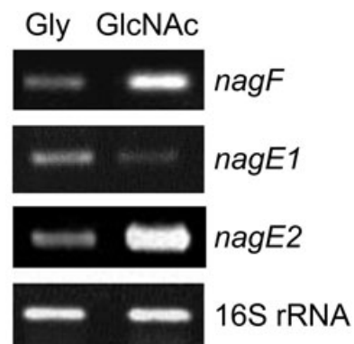
Fig. 4. Transcriptional analysis of the nagF-nagE1-nagE2 locus. Total RNA was prepared from cultures grown on mineral medium supplemented with 50 mM glycerol (Gly) or glycerol plus GlcNAc (GlcNAc). A 1% agarose gel shows RT-PCR amplification products after the 30th cycle of the PCR reaction with oligonucleotides specific for the indicated transcripts. The enhanced expression levels of nagF and nagE2 indicate their GlcNAc-dependent regulation.
