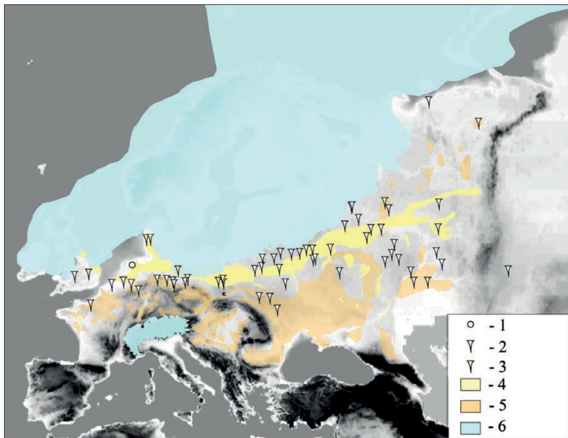
Fig. 3.2. Time window 1: extent of the ice sheet and permafrost indicators at c. 20 kyr BP including the aeolian coversand and loess belt (adapted from Velichko, Zelikson, 2005 and Koster, 2005): 1 – perennial frost mound, 2 – ice wedge cast, 3 – sand wedge, 4 – cover sand, 5 – losses, 6 – ice extent
