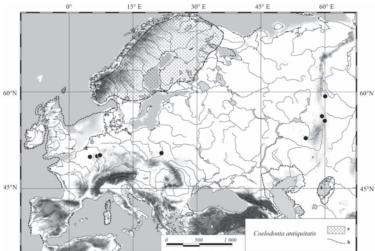
Fig. 4.50. Woolly rhinoceros Coelodonta antiquitatis localities (12.4–10.8 kyr BP); a – ice sheets; b – coastline
