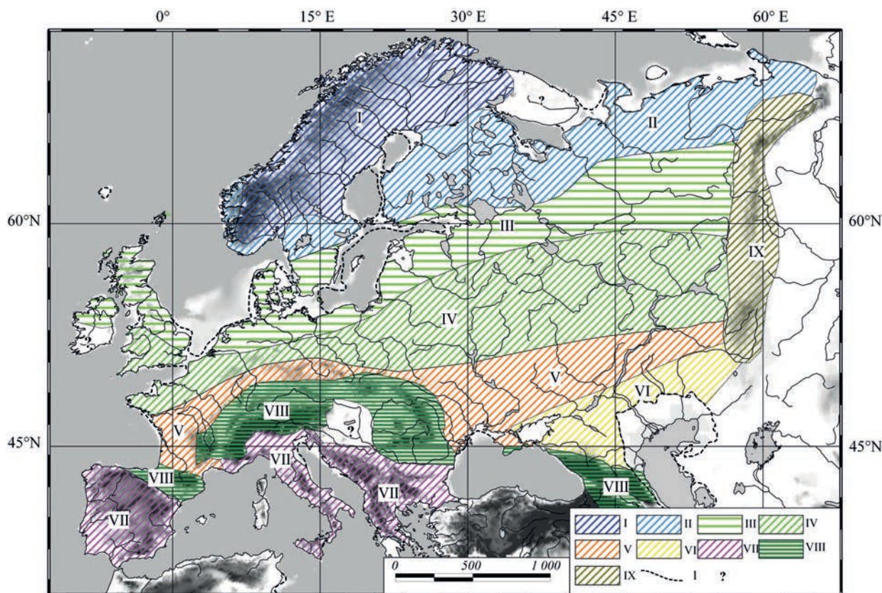
Fig. 6.4. Preboreal-Boreal ecosystems: I – shrub tundra with patches of forest-tundra; II – forest-tundra; III – light pine-birch forests with patches of tundra communities; IV – pine-birch and pine-spruce forest with broad-leaved elements and patches of forest-steppe communities; V – forest-steppe; VI – steppe; VII – Mediterranean xerophytic coniferous-broad-leaved forests with herbaceous communities; VIII – mountain coniferous-broad-leaved forests; IX – The Ural Mountains forest with patches of tundra-steppe communities; ? – absence of data; 1 – coastline
