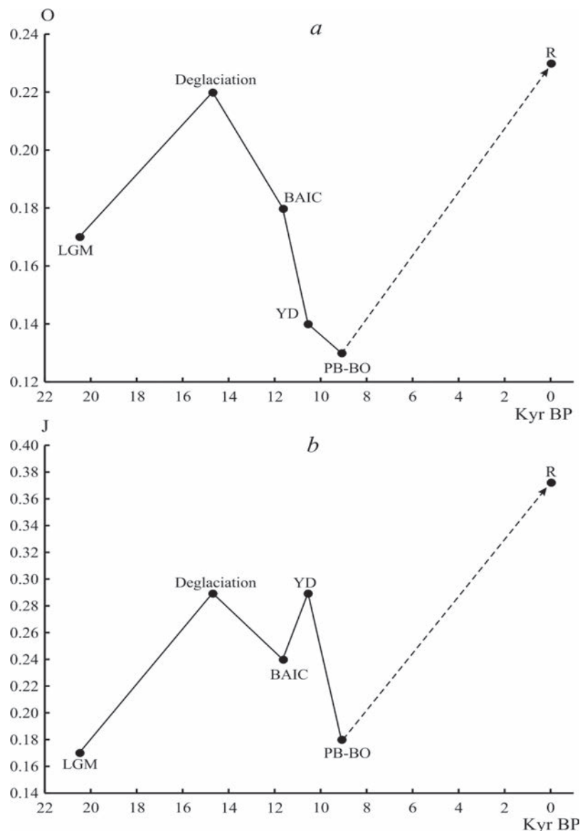
Fig. 4.81. Dynamics of the mammalian species diversity parameters during the transition from the Pleistocene to the Holocene: a (top) – organization measure O ; b (bottom) – Kullback-Leibler measure ( J ). R – the present time
