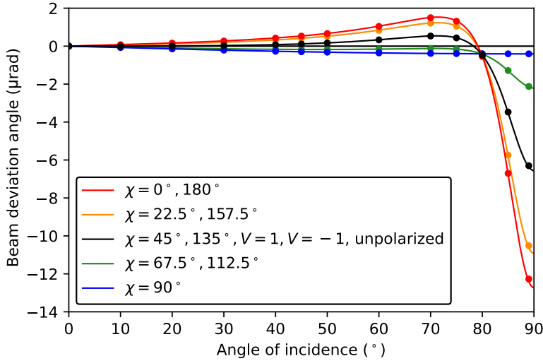
Figure 7.8: Angular GH shift as a function of angle of incidence at a wavelength of 820 nm for a beam of light with an f -number of 61.3 that reflects off gold as obtained from the closed-form expression of Eq. (7.28) (curves) and polarization ray tracing (data points). The shift is shown for an incident beam that is completely unpolarized, 100% linearly polarized with various angles of linear polarization \chi , and 100% right-handed ( V = 1 ) or left-handed ( V = -1 ) circularly polarized.
