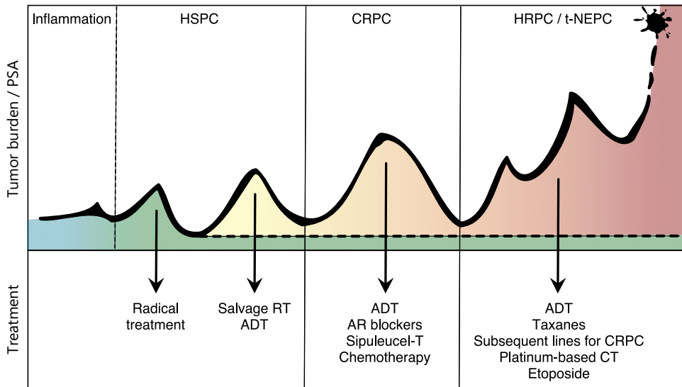
Figure 6 - Prostate cancer natural history
