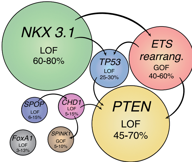
Figure 5 – The genomic landscape of primary PCa
