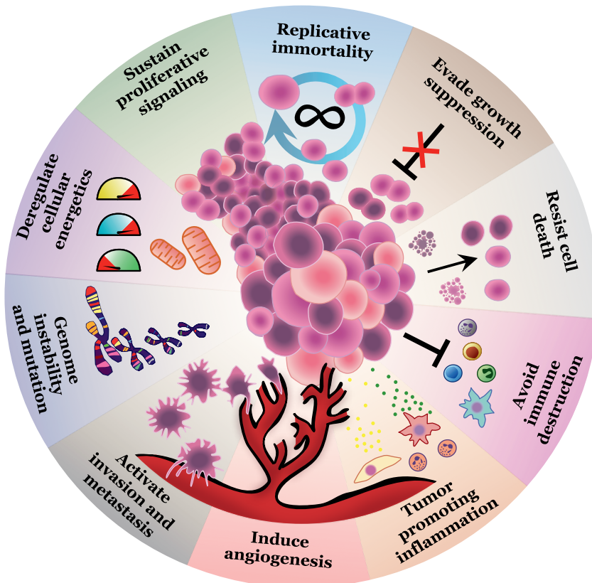
Figure 3 – The hallmarks of cancer, as reported by Hanahan and Weinberg.
