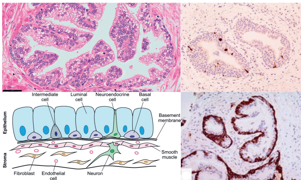
Figure 2 - Prostate histology and cellular components
