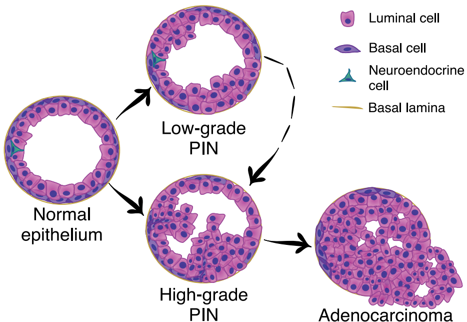
Figure 4 - Prostate cancer formation
