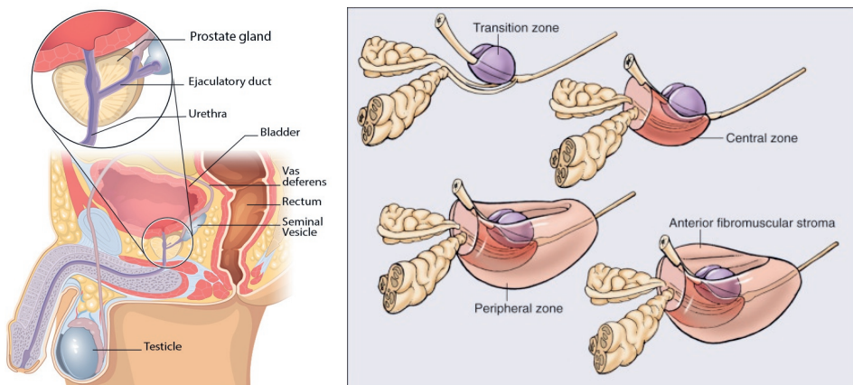
Figure 1. Anatomy of the prostate.
