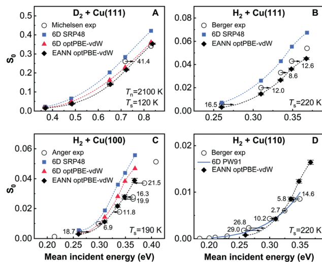
Fig. 39 S_0 computed with PESs based on the optPBE-vdW1 DF for D_2 + Cu(111) (A), H_2 + Cu(111) (B), H_2 + Cu(100) , and H_2 + Cu(110) with high-dimensional QCT calculations are compared with molecular beam sticking experiments 12,649,667,730 on these systems. Black arrows and accompanying numbers (in meV) indicate the incident energy spacing between the experimental and interpolated computed curves. Reproduced from ref. 467 with permission from the PCCP Owner Societies.
