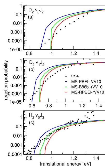
Figure 6. Initial-state-selected reaction probabilities P_{\text{deg}}(E, \nu, J) computed for H_2 ( D_2 ) + Ag(111) using the MS-PBEL-rVV10 (blue), MS-B86bl-rVV10 (green), and MS-RPBE-rVV10 (red) DFs as a function of translational energy are shown, comparing with values extracted from associative desorption experiments. 69,70 Results are shown for D_2 ( \nu = 0, J = 2 ) (a), D_2 ( \nu = 1, J = 2 ) (b), and H_2 ( \nu = 0, J = 3 ) (c).
