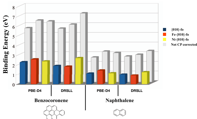
Figure 8. Binding energies of benzocoronene and naphthalene chemisorbed on {010}-fo (singlet), Fe (quintet), and Ni-{010}-fo (triplet) surfaces using PBE-D4 and DRSLL with the CP-DZP basis set and with the corresponding counterpoise-noncorrected values at the back. The order of the labels of the forsterite surfaces corresponds to the order of the bars. Note: Numerical values are reported in the SI.
