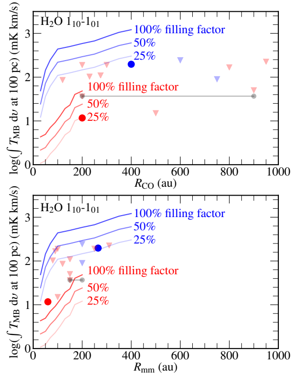
Fig. 29. Line luminosities of models and observations of ortho- H_2O 1_{10}-1_{01} for planet-forming disks observed with Herschel -HIFI. Solid blue and red lines show predicted line luminosities for a Herbig disk model (blue) and a T Tauri disk model (red); see text for details. Note the logarithmic scale. The effects of non-unity filling factors are illustrated by shaded lines at 50 and 25%. The observational data are from Hogerheijde et al. (2011); Du et al. (2017) and Hogerheijde et al. (priv. comm.). Filled circles show detections, blue for the Herbig star HD 100546 and red for the T Tauri star TW Hya. The gray circles connected by the solid gray line show the detected line luminosity of the stacked detection of AA Tau, LkCa15, MWC 480 and DM Tau. Down-pointing triangles show upper limits (blue: Herbig disks; red: T Tauri disks). Data are plotted versus the observed size of the disk as measured through CO emission (upper panel) and mm-wavelength continuum emission (lower panel); for the stacked detection (gray line) the range of disk sizes is plotted. Observed disk sizes are taken from Walsh et al. (2014); Andrews et al. (2012); Loomis et al. (2017); Bergin et al. (2016); Kudo et al. (2018); Jin et al. (2019); Qi et al. (2003); Liu et al. (2019); Fedele et al. (2017); Huang et al. (2016); Dutrey et al. (2003, 2016); Hughes et al. (2009); Macías et al. (2018); Isella et al. (2016); Boehler et al. (2018); Huélamo et al. (2015); Cleeves et al. (2016). Line luminosities and disk sizes are scaled to the latest Gaia distance estimates.
