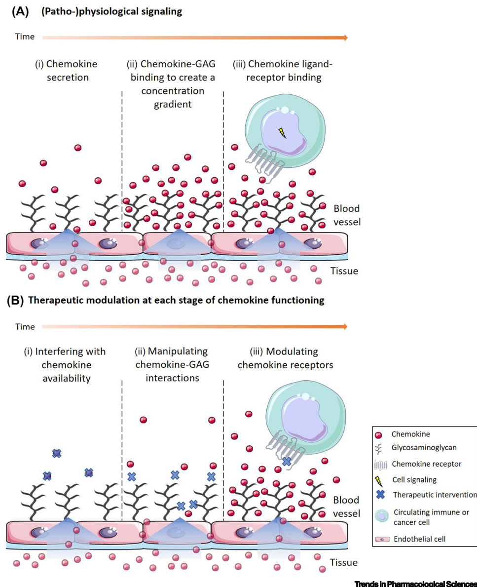
Figure 1. Avenues for therapeutic intervention in chemokine ligand-receptor signaling. (A) Schematic visualization of the steps involved in chemokine ligand-receptor signaling over time. (i) chemokine secretion; (ii) chemokine-glycosaminoglycan (GAG) binding to create a concentration gradient; and (iii) chemokine ligand-receptor binding. (B) Schematic visualization of how therapies can interfere with these steps. Therapies can: (i) intervene with chemokine availability; (ii) prevent chemokines from binding to GAGs and thus, precluding a chemokine gradient; or (iii) block chemokine receptors to prevent chemokine binding and (oncogenic) downstream signaling. This figure was created using elements from Servier medical art.
