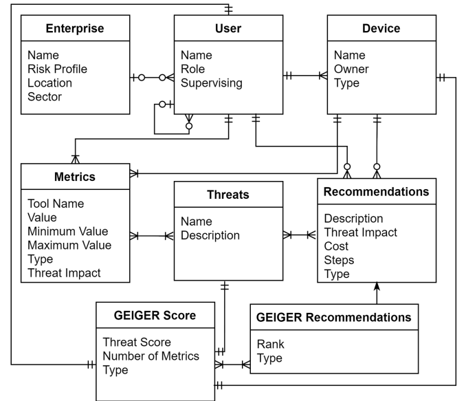
Figure 2: The conceptual data model underlying our threat-based cybersecurity risk assessment approach.
