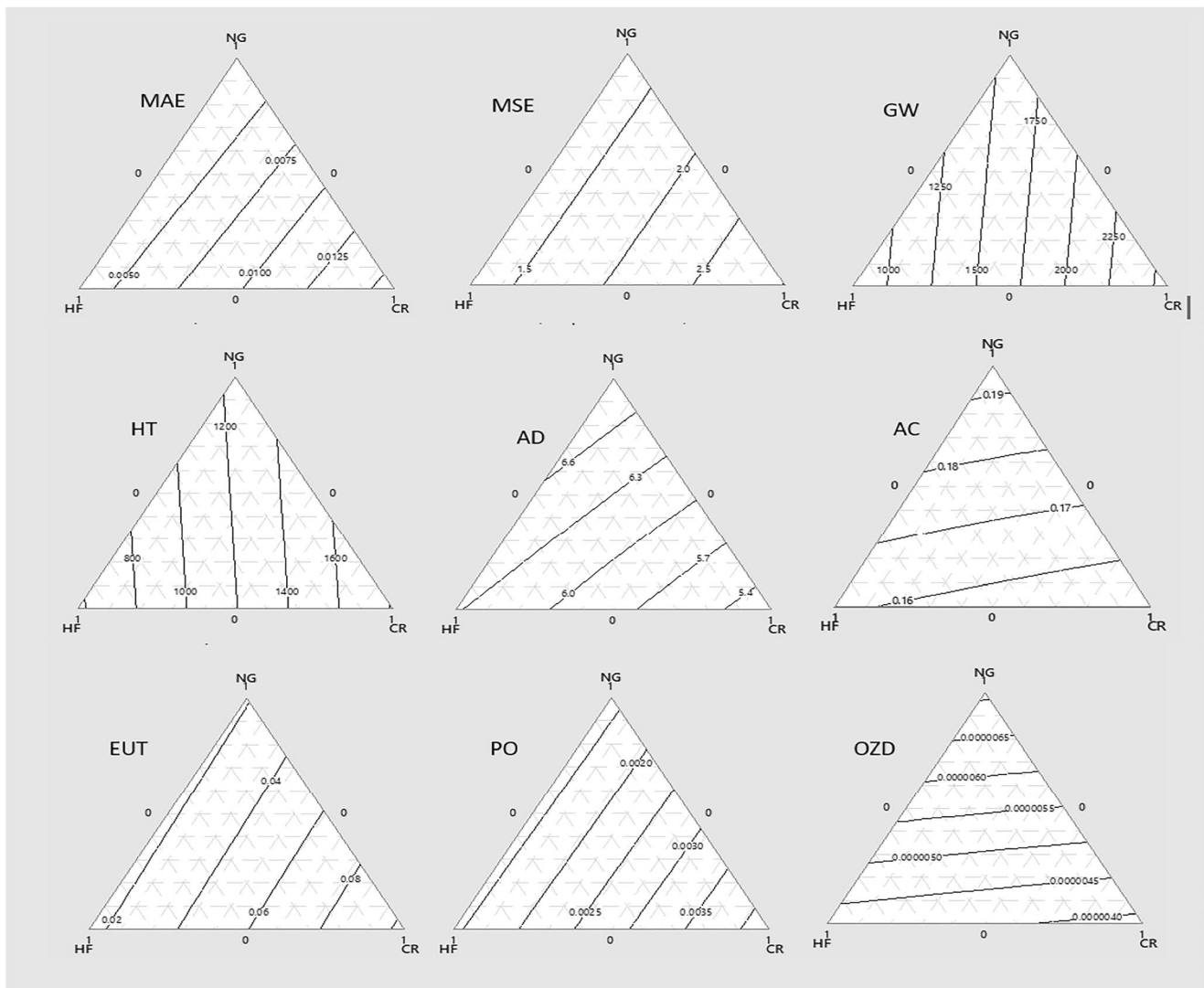
Fig. 4 Mixture contour plot for LCIA, with GO held constant at zero, shown in fossil fuel proportions to desalinate 1 \text{ m}^3 of seawater, derived using regression equations
