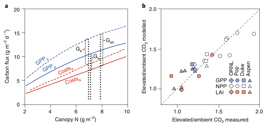
Fig. 1 | Optimality model of \text{CO}_2 and N availability effects in FACE experiments. a , The hypothesis is that trees optimize canopy N (vertical dashed lines) by maximizing net C gain ( G = \text{GPP} - \text{costs} ), where costs are carbon costs for maintaining the canopy (respiration + leaf and root turnover). Elevated \text{CO}_2 (subscript e) increases GPP compared to ambient \text{CO}_2 (subscript a), causing a potential large increase in optimal canopy N and net C gain ( G_{eh} ), which is not realized due to a simultaneous increase in C costs per N uptake (due to soil N limitation), resulting in a smaller net effect ( G_e ). b , Modelled versus measured \text{CO}_2 effects on productivity (GPP and NPP) and leaf area index (LAI) in forest FACE experiments with sweetgum (ORNL), loblolly pine (Duke), poplar (Pop) and aspen. r^2 = 0.83 . Adapted from ref. 20 .
