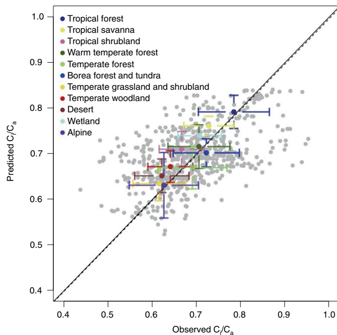
Fig. 2 | \text{CO}_2 uptake parameters predicted by an optimality principle. Using uniform parameters in conjunction with a cost-minimizing optimality hypothesis, a theoretical model predicts the ratio of leaf-internal to ambient \text{CO}_2 ( C_i/C_a )—a key index of leaf-level C and water exchange—across the world's biomes 23 . The inputs are growing season temperature, vapour pressure deficit and elevation. Observations (based on leaf \delta^{13}\text{C} data) are compared with model predictions. Means and standard deviations are indicated for each biome. Although there is considerable unexplained variation among individual plants (grey points, r^2 = 0.26 ), biome means are well predicted by the model ( r^2 = 0.72 ). The continuous line represents the regression line (constrained to pass through the origin); the dashed line represents the 1/1 line.
