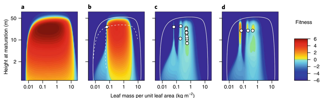
Fig. 3 | Modelling diverse communities based on evolutionarily stable strategies. By modelling reproductive success in competition with existing types (white dots), ESS models estimate the fitness of potential invaders (coloured shading) and use this to guide community assembly. Here, species are allowed to vary in two traits, underpinned by physiological trade-offs. a , Initially, a wide variety of trait combinations have positive fitness and could establish. b , Through directional selection, any single species is driven towards a local evolutionary attractor. However, this single species cannot prevent the invasion of other types if regions of positive fitness occur elsewhere in trait space. c , Through repeated rounds of mutation and selection, an ESS trait mixture may be established—that is, existing residents all have positive abundance while fitness is zero or negative elsewhere. The ESS trait mixture represents a prediction for the system diversity. d , In traditional models with pre-specified trait combinations, species may coexist but are not evolutionarily stable—that is, they could be invaded if new plant types were allowed into the system. In each panel, the solid white line delimits trait combinations that are not viable even in the absence of any competition (pure environmental filtering, as indicated in a ). In b , the dashed white line shows the evolutionary attractors for each trait when allowed to evolve in isolation 68 .
